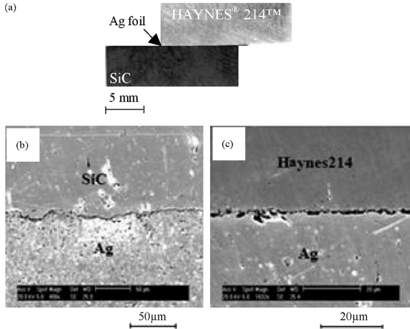
Fig. 7. Cross-section of SiC/Ag/HAYNES ® 214 ™ joint. (a) Optical macrograph of the no reactive zone. Cross-sectional Scanning Electron Micrograph of the SiC/Ag/HAYNES ® 214 ™ joint, (b) SiC/Ag interface, and (c) HAYNES ® 214 ™ /Ag interface.
