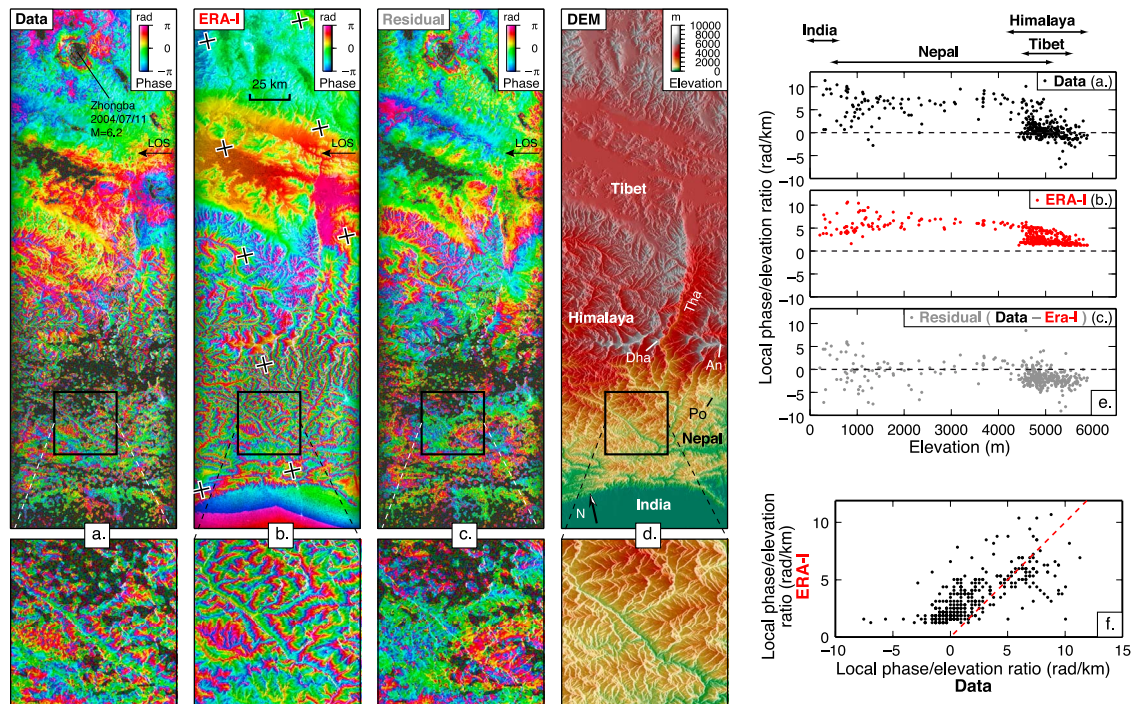
Figure 3. Example of interferogram and atmospheric correction across the Himalaya. (a) Wrapped interferogram from SAR acquisitions on 17-03-2004 and 08-09-2004, in radar geometry. (b) Corresponding stratified delay map predicted from ERA-I data. Dark crosses are ERA-I grid locations. (c) Residual after subtraction of Figure 3b from Figure 3a. (d) SRTM digital elevation model (DEM). Dha: Dhaulagiri (8167 m); An: Annapurna I (8091 m); Po: city of Pokhara; Tha: Thakkhola graben. Inset below each map shows a blowup of the region indicated by the black squares. (e) Observation (top, black), full-grid ERA-I prediction (middle, red) and residuals after ERA-I correction (bottom, grey) for local phase/elevation ratios computed in moving windows spanning the wrapped interferograms. Dashed line shows zero mean phase/elevation ratio. (f) Observed (x-axis) versus predicted (y-axis) phase/elevation ratios computed in each moving window in interferograms in Figures 3a and 3b, respectively. The red dashed line indicates the unit correlation. Correlation coefficient is 0.67.
