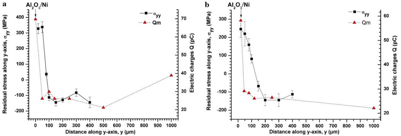
Fig. 11. Comparing the quantity of influence charges Q_m and residual stress estimated by Vickers indentation in both types of assemblies: (a) \text{Al}_2\text{O}_3/\text{Ni}/\text{HAYNES}^{\text{TM}}214 , (b) \text{Al}_2\text{O}_3/\text{Cu}_2\text{O}-\text{Cu}/\text{Ni}/\text{Cu}/\text{HAYNES}^{\text{TM}}214 .
