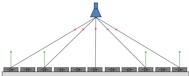
Figure 1. Antenne reflectarray reconfigurable
