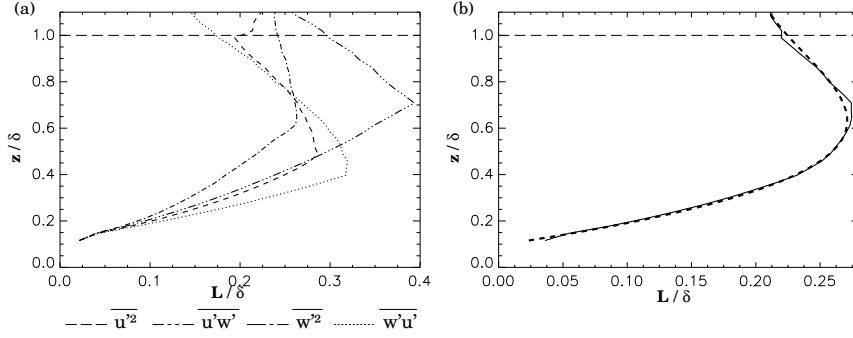
FIGURE 4 – (a) : Integral length normalized by \delta for \overline{u'^2} (dashed lines), \overline{w'^2} (dash-dot lines), \overline{u'w'} (dash-dot-dot line) and \overline{w'u'} (dotted lines) following the vertical direction. (b) : Mean experimental integral length scale ( L ) (solid line) and its fit (dashed line).
