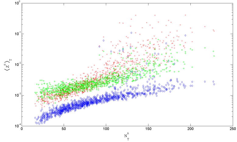
FIG 2. " \times ", " + " and " \diamond " correspond respectively to " \langle Z^n \rangle_{T, uniform} ", " \langle Z^n \rangle_{T, fractional} " and " \langle Z^n \rangle_{T, stochastic} ".
