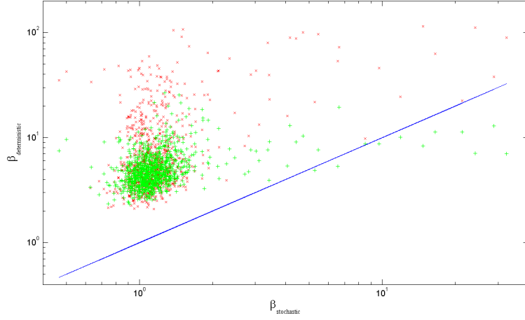
FIG 1. " \times ", " + " and the blue line correspond respectively to " (\beta_{stochastic}, \beta_{uniform}) ", " (\beta_{stochastic}, \beta_{fractional}) " and the identity function.
