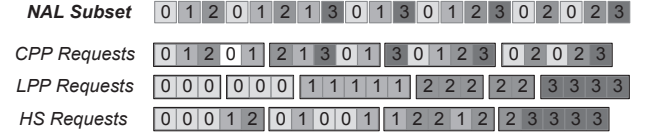
Figure 7: Generated requests for the three pull approaches.
