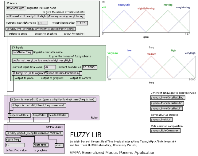
Figure 2. A screenshot of the help patch of the ‘ gmpa ’ object (Generalized Modus Ponens Application) connecting two linguistic variables ( qom and freq ) and taking into account fuzzy rules.
