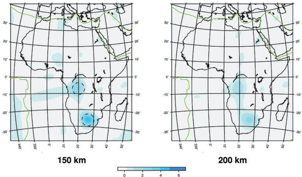
Figure A3. Results of a second synthetic resolution test in which we insert two 750-km-diameter, 200-km-thick discs, having a 5 per cent positive velocity perturbation, centred at 7.5°S, 20°E and 27.5°S, 27.5°E (dashed circles in 150 km map). The result at 150 km depth shows substantial smearing of the high anomaly, centred at 7.5°S, 20°E westward into the Gulf of Guinea but minimal smearing occurs at 200 km depth.
