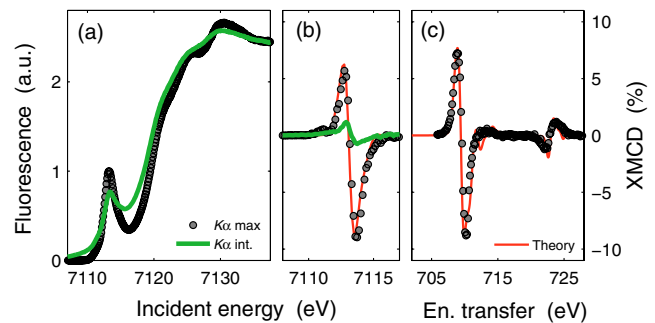
FIG. 2 (color online). Line scans extracted from the RIXS-MCD plane. Comparison of the Fe K edge spectra (a) and their magnetic circular dichroism (b) acquired at the maximum of K\alpha_1 fluorescence line (dots) and using the K\alpha_{1,2} -integrated spectrum [thick (green) line]. The K\alpha_1 -detected XMCD spectrum shows almost eightfold enhancement of the dichroism as compared to K\alpha_{1,2} -integrated and is in good agreement with the theoretical spectrum [thin (red) line]. (c) Comparison between theoretical [thin (red) line] and experimental (dots) XMCD spectra acquired at constant incident photon energy, which corresponds to a vertical line through the RIXS-MCD plane at the incident energy of 7113.6 eV. The measured XMCD effect shown in (b) and (c) is relative to the maximum preedge intensity, while the intensity of the theoretical XMCD is scaled down by factor of 5.67 to obtain best match.
