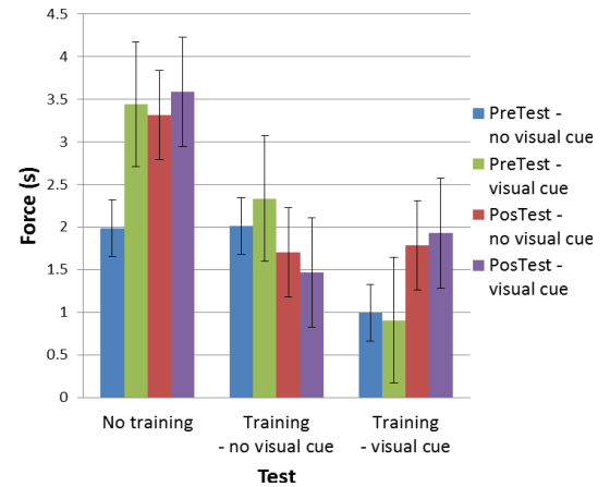
Fig. 6: Average Maximum Force
