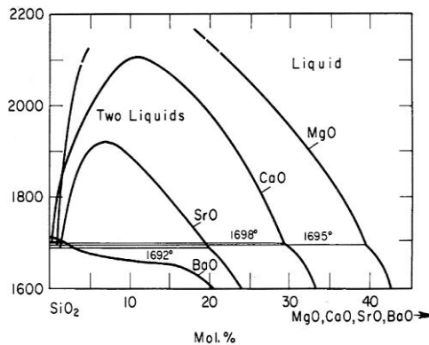
Fig. 12: Immiscibility-gap in the phase-diagram of binary \text{SiO}_2\text{-MO} glass ( M = \text{Mg, Ca, Sr} )
