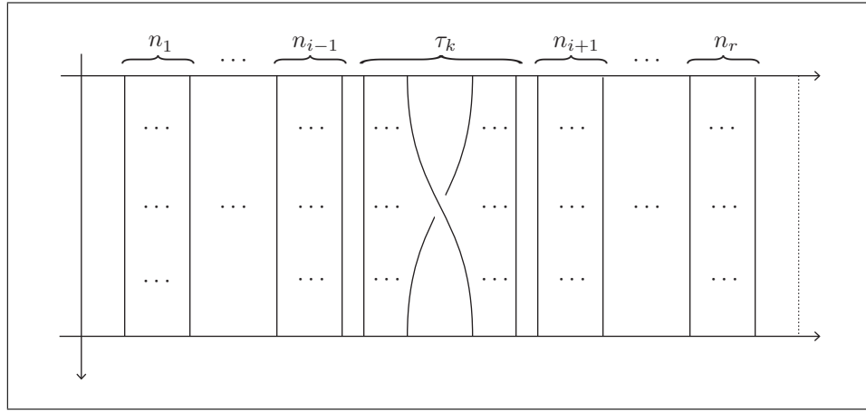
FIGURE 2.7. The direct sum id \oplus \dots \oplus \tau_k \oplus \dots \oplus id in the braid group.
