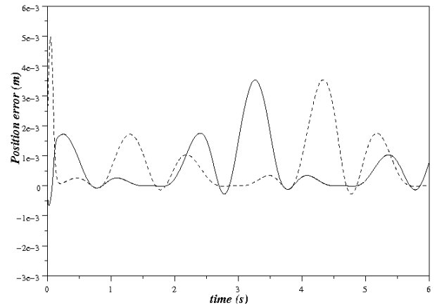
Fig. 9. Position error between actual and desired position: on \vec{i} -axis (solid), on \vec{k} -axis (dotted)
