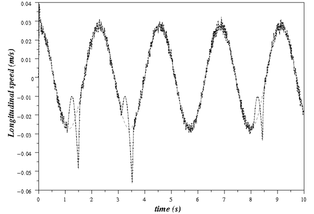
Fig. 5. Longitudinal speed: reference speed (grey dots), actual speed (black dots) and estimated speed (grey solid line)
