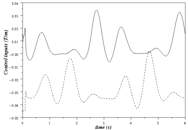
Fig. 10. Control inputs: magnetic field gradients on \vec{i} -axis (solid), on \vec{k} -axis (dotted)
