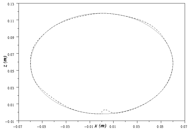
Fig. 8. XY trajectory: reference trajectory (grey) and actual trajectory (black dotted)
