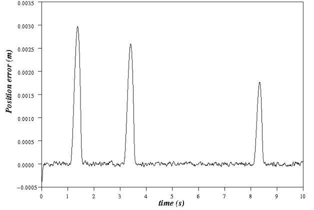
Fig. 4. Error between actual and reference position
