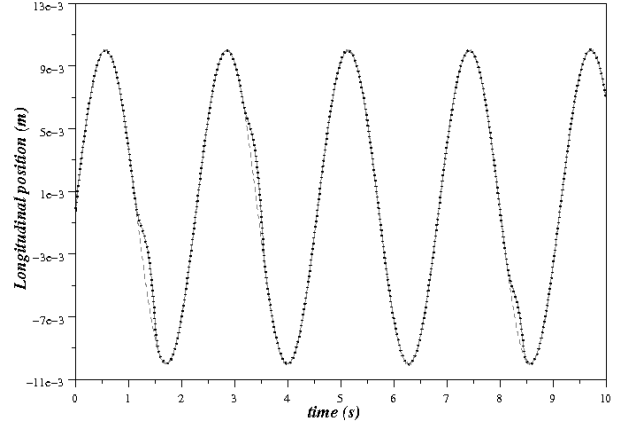
Fig. 3. Longitudinal position: reference position (grey dots), actual position (black dots) and estimated position (grey solid line)
