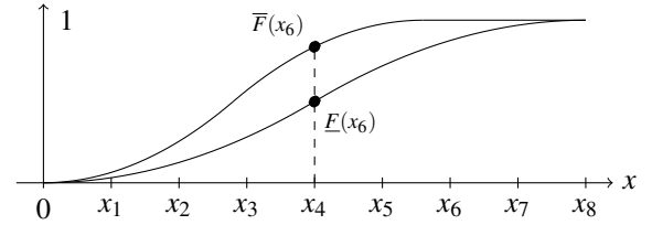
Figure 4: Discretisation of a f-filter with 8 sampled values
