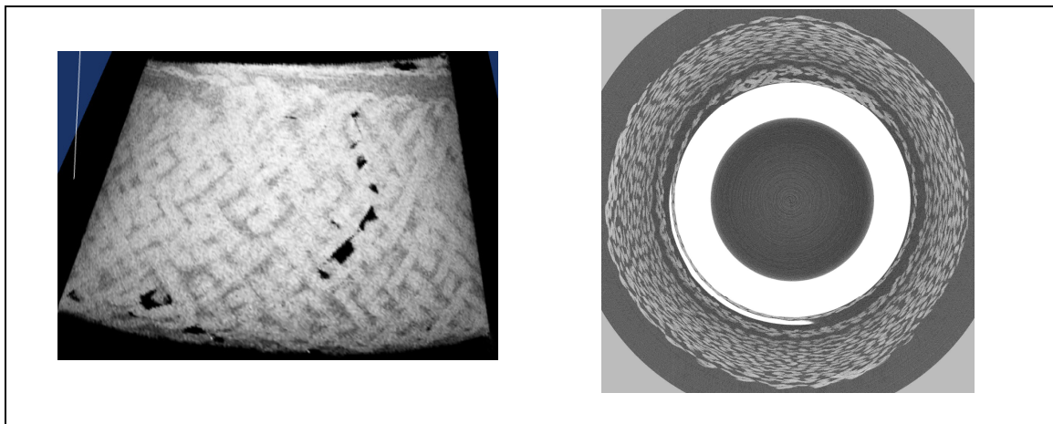
Fig. 2 (a) Position of yarns on a ply; (b) tomography to estimate the density
