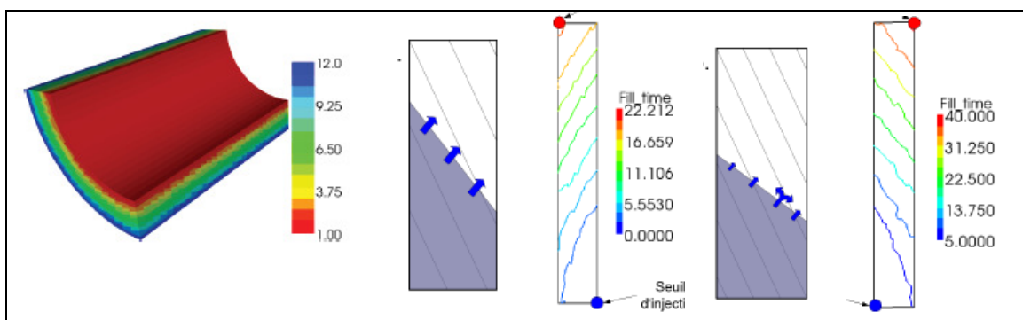
Fig. 4. Simulation. (a) Definition of material. (b) V_f constant .(c) V_f not constant.
