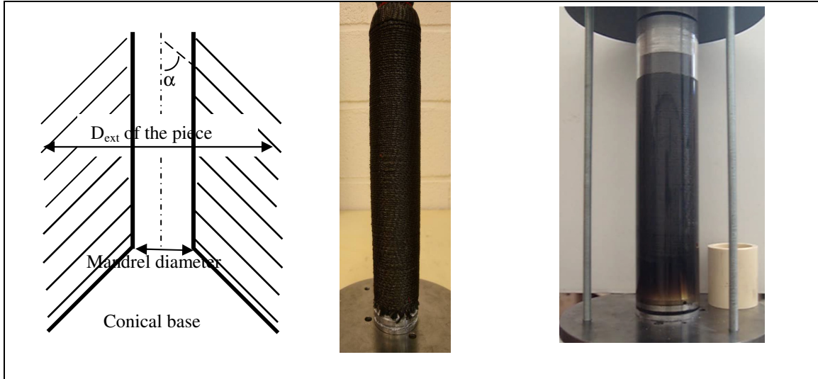
Fig. 1 (a) Scheme of the preform; (b) Final preform; (c) Resin evolution
