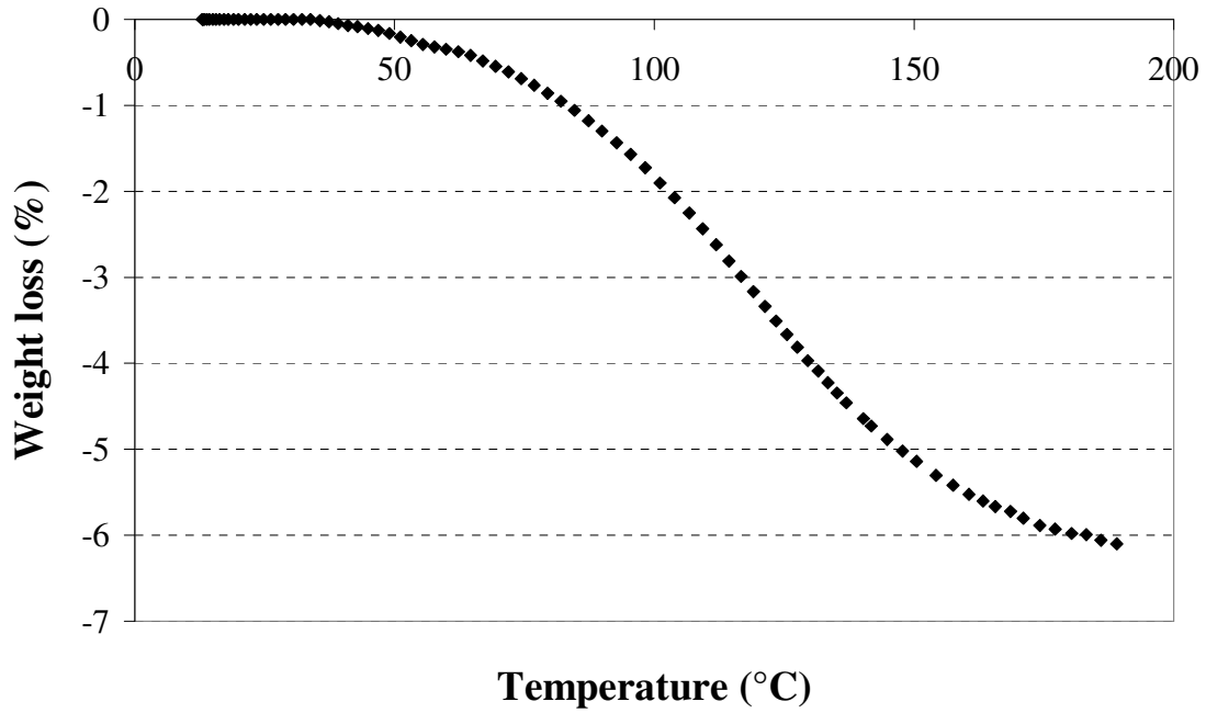
Figure 9: Influence of the increasing temperature upon the weight loss of flax fibres
