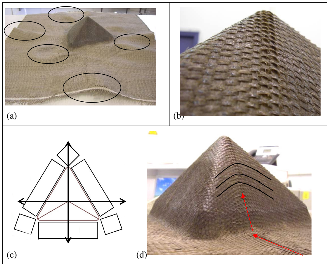
Figure 2: (a) Preform and Wrinkles. (b) Zoom on buckles. (c) Position of buckles. (d) yarns orientation
