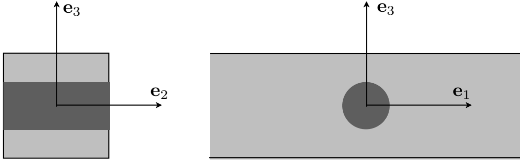
Fig. 7 Unidirectional reinforcements
