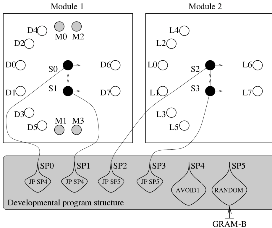
Figure 12. The initial configuration of the developmental substrate and the program structure used in Stage 2 for the evolution of obstacle-avoidance in Khepera. The same substrate was used for control experiments, in which both modules were evolved simultaneously. In these latter experiments, both SP4 and SP5 were initialized randomly and were submitted to evolution under constraints given by GRAM-A and GRAM-B, respectively.
