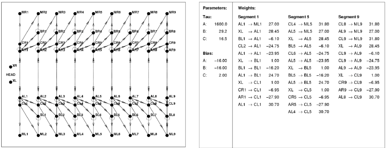
Figure 27. Architecture of controller 10, one of the two controllers producing anguiform swimming. Left: Neurons on the substrate. For the sake of clarity, the lateral axis of the substrate has been multiplied by ten. ML_i and MR_i represent the left and right muscle nodes of segment i ; X_L and X_R are the input nodes. A, B and C are three types of neurons. Excitatory and inhibitory connections are represented through continuous and dashed lines respectively. Each neuron also receives a connection from the input nodes, which is not shown here. Right: Parameters and connection weights. Only the weights of the connections to the left neurons are given, the others are symmetrical.
