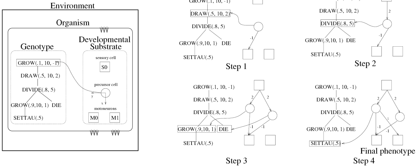
Figure 3. The developmental encoding scheme of SGOCE. The genotype that specifies the animat's nervous system is encoded as a grammar tree whose nodes are specific developmental instructions. Within such chromosomes, mutations change one branch into another, and crossovers swap branches. Each cell in the developing network reads the chromosome at a different position. The number of developmental steps required to generate a phenotype varies depending upon the length of the corresponding genotype.
