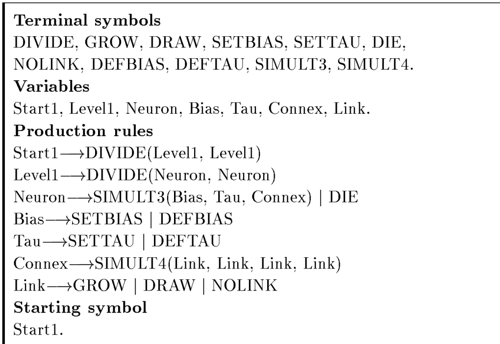
Figure 10. The GRAM-A grammar, according to which a cell undergoes two division cycles yielding four daughter cells, which can either die or modify internal parameters (time-constant and bias) that will influence their future behavior as neurons. Each surviving cell establishes a maximum number of four connections, either with another cell or with sensory cells and motoneurons.
