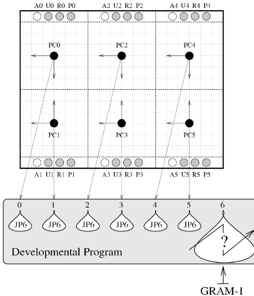
Figure 2. Setup for the evolution of a neural network that will be used in section 4 to control locomotion in a six-legged animat. The figure shows the initial positions of the sensory cells, motoneurons and precursor cells within the substrate, as well as the structure of the developmental programs that call upon seven subprograms. JP is a call instruction that forces a cell to start reading a new subprogram. Only subprogram 6 needs to be evolved. Its structure is constrained by the GRAM-1 tree-grammar (to be described in section 2.B). Additional details are to be found in the text.
