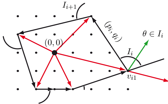
FIGURE 6. The Polygon \text{Pol}_S^0 for a surface S negatively transverse to the geodesic flow. For a \gamma -regular angle \theta , the directions [S_\theta] (indicated by a red arrow) and \theta (indicated by a green arrow) form a direct basis. The point (0,0) is on the left of all edges of \text{Pol}_S^0 , and therefore in the interior or on the boundary of \text{Pol}_S^0 .
