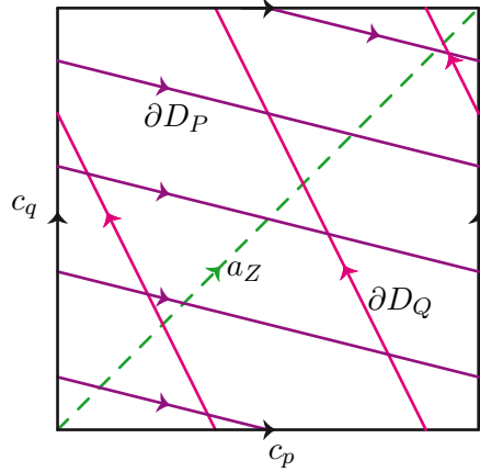
FIGURE 17. The median torus \overline{T^1 e} , in the basis (c_p, c_q) , here with p = 5 and q = 3 . The hyperbolic compactification \overline{T^1 \Sigma_{p,q,\infty}} is obtained by gluing two solid tori \overline{T^1 \Delta_P / \Gamma_P} and \overline{T^1 \Delta_Q / \Gamma_Q} , with respective meridian \partial D_P and \partial D_Q , along \overline{T^1 e} . The fibers of the points of e are the curves on \overline{T^1 e} that are parallel to a_Z .
