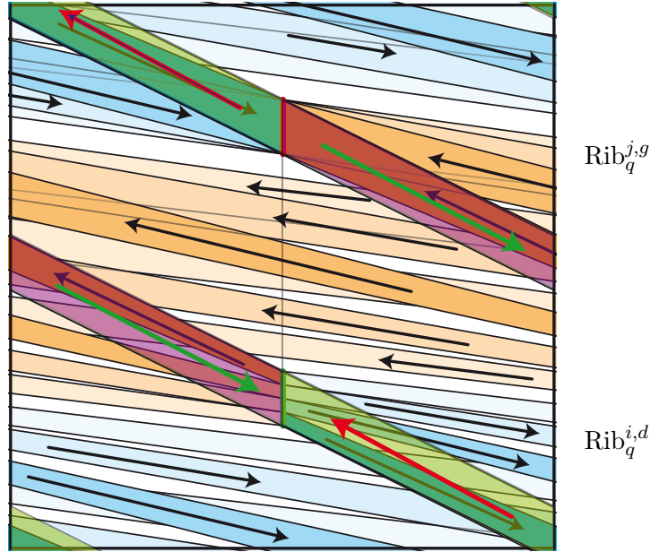
FIGURE 19. The two projections of \mathcal{B}_{\Gamma_{2,q},\mathcal{T}_{P,Q}} on \overline{T^1e} , with q = 5 , in the slide-of-cake model. The curve a_Z is the vertical boundary of the depicted square, while the curve c_Q is the horizontal boundary. The solid torus T^1\Delta'_P/\Gamma_P is in front of the picture, so that we see on the front the two projections of the ribbon \text{Rib}_p . On the back, the two projections of each of the four ribbons \text{Rib}_q^1, \dots, \text{Rib}_q^4 .
