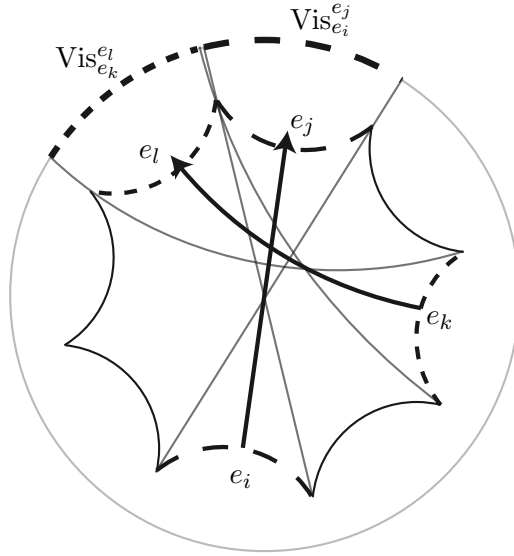
FIGURE 10. The visual intervals \text{Vis}_{e_i}^{e_j}, \text{Vis}_{e_k}^{e_l} associated to two intersecting edges of \mathcal{G}_\mathcal{T} . Since \text{Vis}_{e_i}^{e_j} and \text{Vis}_{e_k}^{e_l} are disjoint, the associated ribbons \text{Rib}_{e_i}^{e_j}, \text{Rib}_{e_k}^{e_l} do not intersect.
