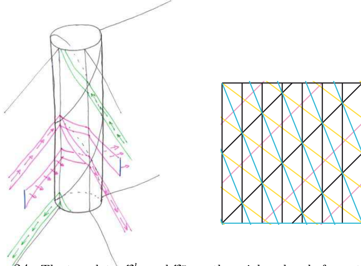
FIGURE 24. The templates \mathcal{B}_{14}^l and \mathcal{B}_{14}^r on the neighbourhood of a vertex V_i . For \mathcal{B}_{14}^l , most of the ribbons go down by 10\pi/14 (in blue), or they are close to a branching segment and they go down by 3\pi/14 (in yellow), unless they are close to both branching segments and they go up by 4\pi/14 (in pink). For \mathcal{B}_{14}^r , the signs are reversed.
