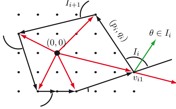
FIGURE 6. The Polygon \text{Pol}_S^\circ for a surface S negatively transverse to the geodesic flow. For a \gamma -regular angle \theta , the directions [S_\theta] and \theta form a direct basis. The point (0,0) is on the left of all edges of \text{Pol}_S^\circ , and therefore in the interior or on the boundary of \text{Pol}_S^\circ .
