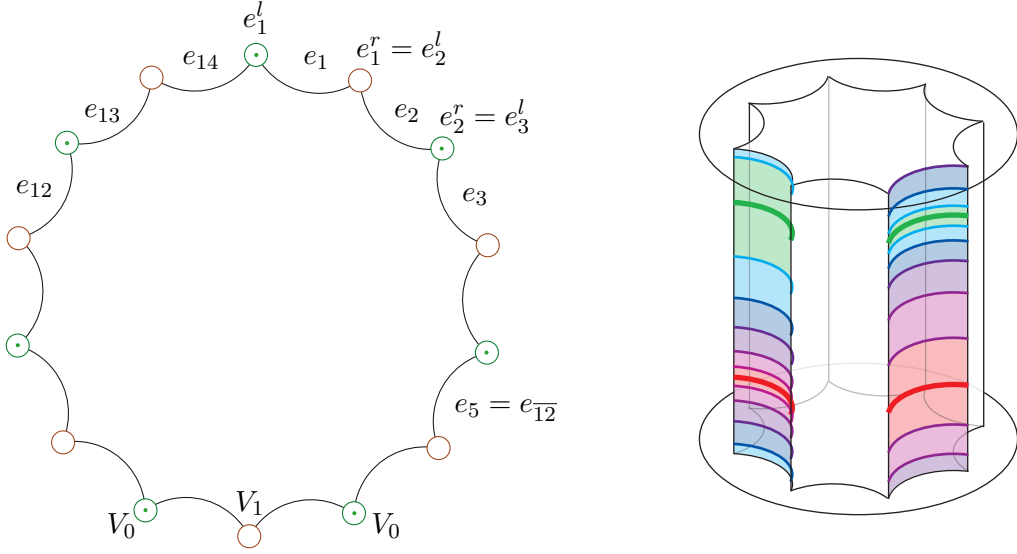
FIGURE 21. On the left, the regular 14-gon P_{14} . The surface \Sigma_3 is obtained by identifying opposite sides. The unit tangent bundle is obtained in the standard coordinates P_{14} \times \partial_\infty \mathbb{H}^2 by gluing opposite walls using homographies (on the right of a genus 2 surface).
