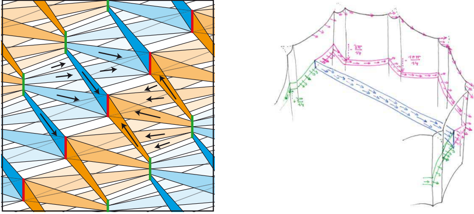
FIGURE 22. On the left, the template \mathcal{B}_{14} (with 5 instead of 14) projected on T^1\partial P_{14} . On the right, a ribbon \text{Rib}_{i,j}^l and its projection \text{Rib}_{i,j}^l on T^1\partial P_{14} . By definition, it is horizontal in every wall of type T^1e_i . As stated in Lemma 6.8, it goes down around every vertex. This long descent (which is reminiscent of a picture by Escher) stems from the observation that a vector travelling along the left boundary of P_{14} and staying tangent to \partial P_{14} has to turn right at every vertex.
