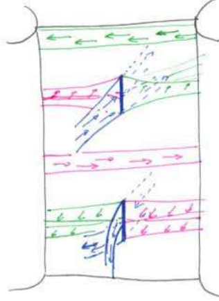
FIGURE 23. The templates \mathcal{B}_{14}^l and \mathcal{B}_{14}^r inside a wall of type T^1 e_i . Between the two branching segments, all ribbons have the same orientation. If \gamma is a null-homologous collection of orbits of \mathcal{B}_{14} , then there are as many arcs of \gamma_\pi traveling from left to right (along the pink ribbons) as arcs of \gamma_\pi traveling from right to left (along the green ribbons).
