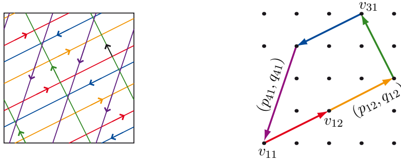
FIGURE 2. A null-homologous family \gamma of periodic orbits of the geodesic flow, and the associated polygon \text{Pol}_\gamma .
