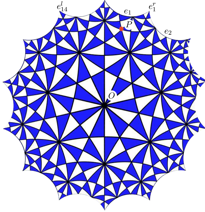
FIGURE 25. The covering of the orbifold \Sigma_{2,3,7} by the genus 3-surface \Sigma_3 .
