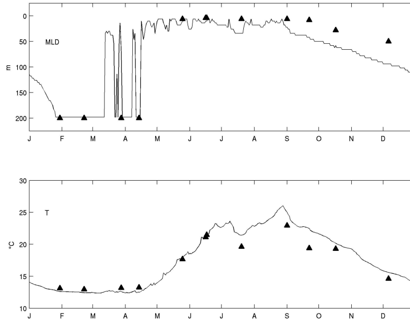
Annual time course of the mixed layer depth and 5 m depth temperature for the model (line) and the observations (triangles). Mixed layer depth observations are bounded at 200m, the bottom of the modeled domain.
