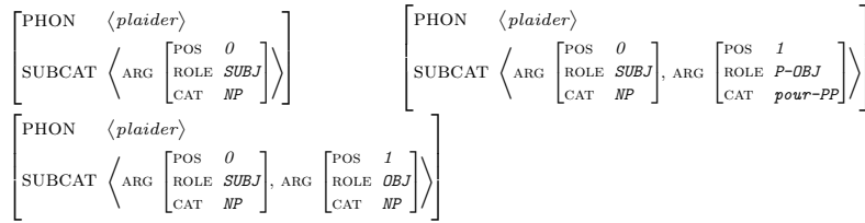
Fig. 1. Subcategorisation schemes for the verb plaidier (to plead).
