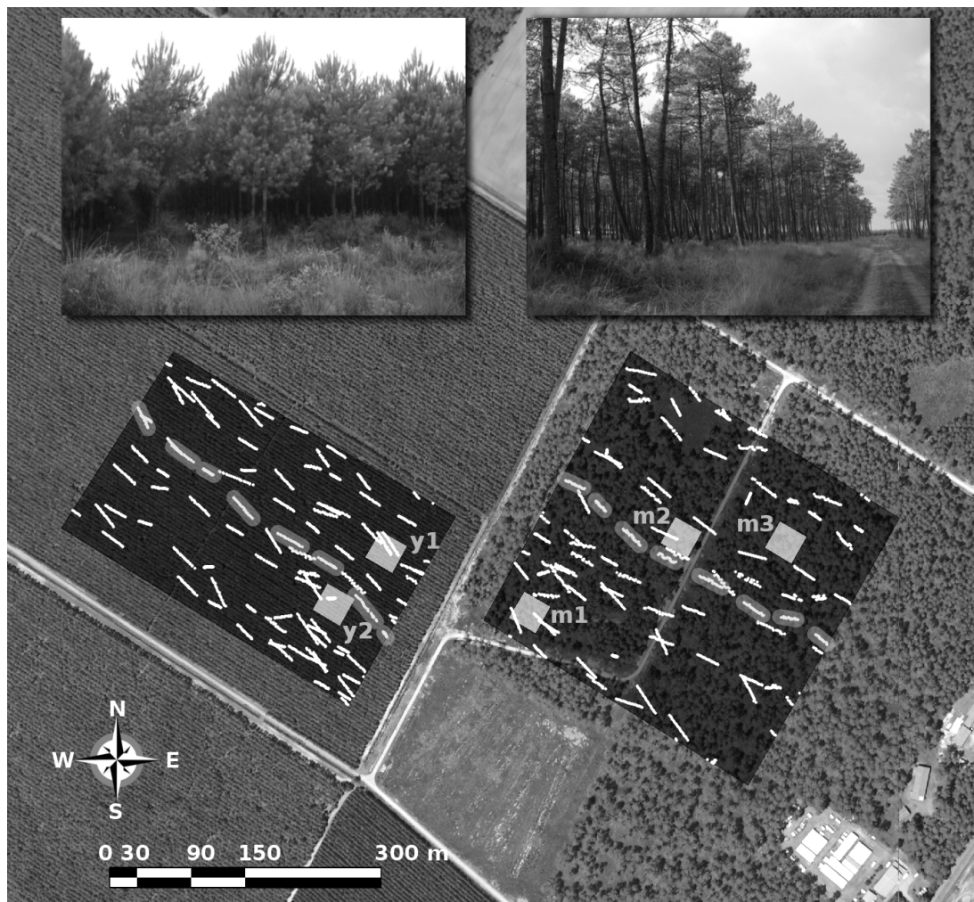
210 Fig. 2. The study area. The white dots represent the lidar shoots falling inside the young stand (west) and the mature stand (east). The enlighten dots (gray) represent lidar shoots of a unique 215 flight line. The light-gray squares represent the locations of the terrain plots (young plots: y1 and y2. mature plots: m1, m2 and m3).
