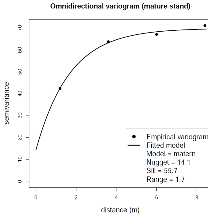
535 Fig. 6. Omnidirectional variogram for the mature, semi-natural stand.
