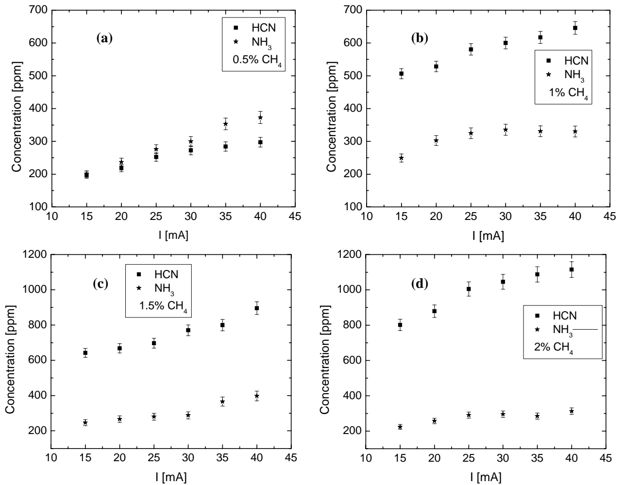
Figures 3. The dependence of HCN and \text{NH}_3 concentrations on the discharge current for different initial \text{CH}_4 concentrations (a - 0.5; b - 1; c - 1.5; and d - 2%) in \text{N}_2 plasma.
