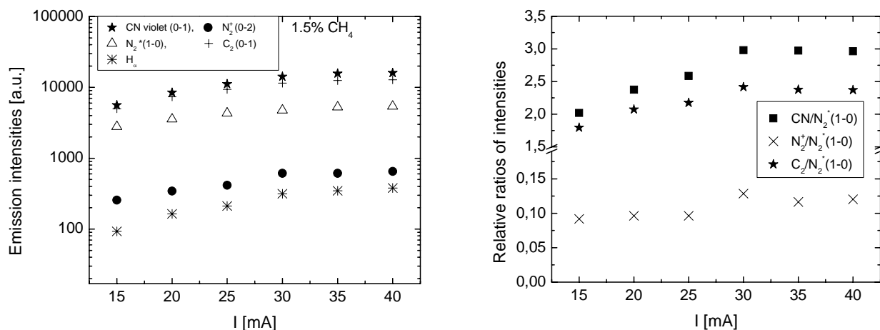
Figures 5. Emission intensities and ratios for the selected emission bands in a gas mixture of 1.5% CH 4 in N 2 .
