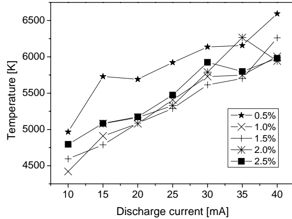
Figures 7 (6). Dependence of N_2^+ and CN vibrational temperatures on the discharge current for various CH_4 content.
