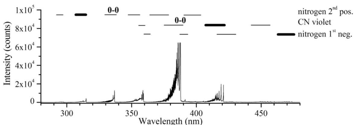
Figure 4. A portion of the emission spectrum recorded using a discharge current of 40 mA and 2.0 % CH 4 content in N 2 . Components of several emission bands are labeled.
