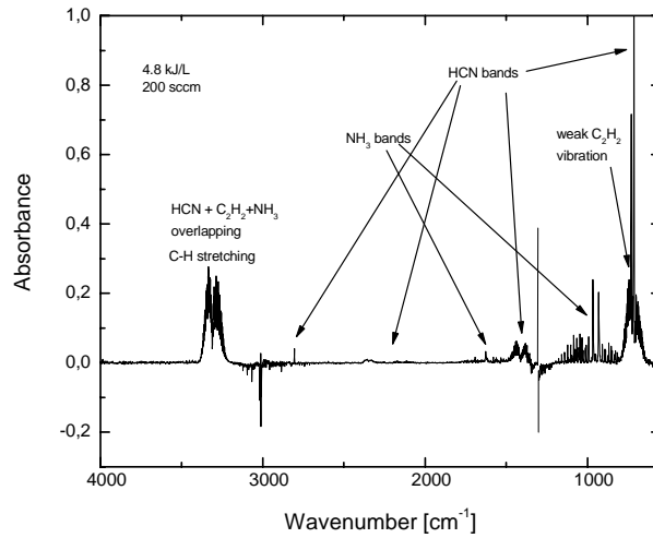
Figure 2. A typical FTIR spectrum recorded in a gas cell filled with products formed in the discharge reactor fed by a \text{CH}_4\text{-N}_2 gas mixture with a 2:98 ratio, operated at atmospheric pressure and a total gas flow 200 sccm. The unit energy has a value of 4.8 kJ/L. Note the negative absorbance indicates the conversion of \text{CH}_4 during the operation of the discharge
