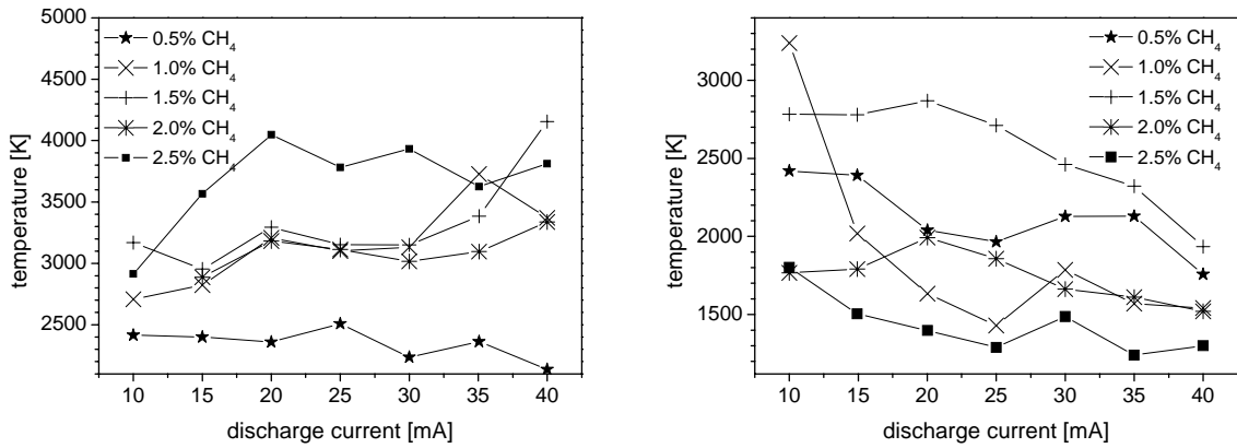
Figure 6. Rotational temperatures calculated from the nitrogen second positive (left) and CN violet (right) 0-0 bands.
