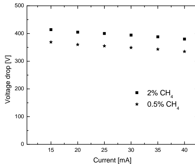
Figure 9. Current-Voltage characteristics in \text{CH}_4/\text{N}_2 plasma for 0.5 and 2% \text{CH}_4 content.
