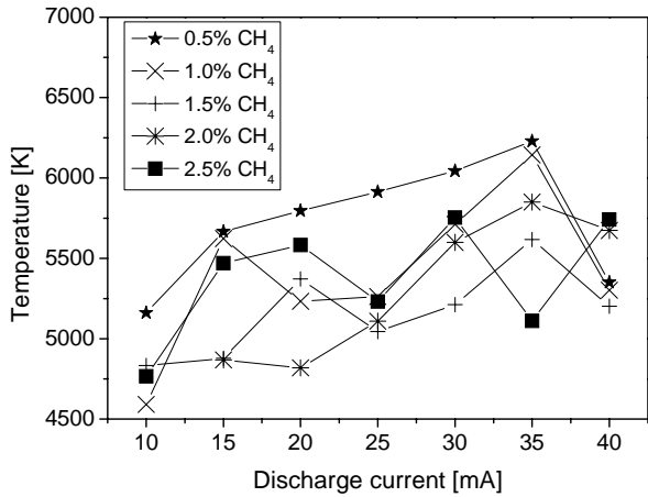
Figures 7 (6). Dependence of N_2^+ and CN vibrational temperatures on the discharge current for various CH_4 content.
