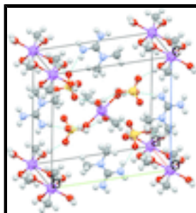
Fig. 2. Molecular packing, showing intermolecular hydrogen bonding interactions (blue lines) as viewed along the a axis.
