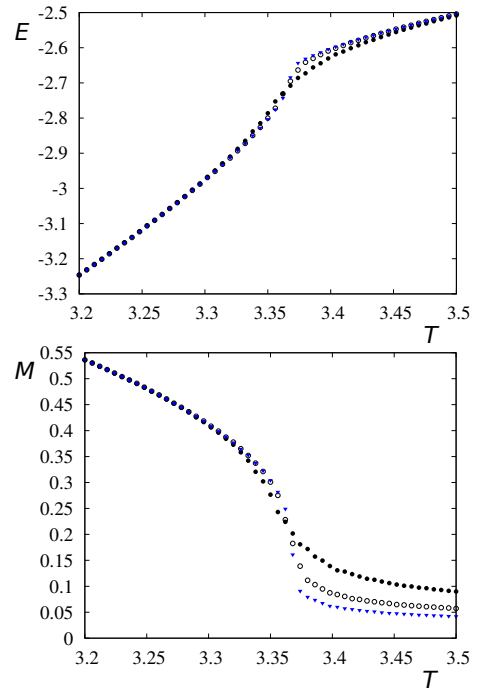
FIG. 6. Internal energy per spin E and order parameter M = \langle Q \rangle versus T for D = 2 , r_c = \sqrt{10} with several lattice sizes N_z = N = 24 (black circles), 36 (void circles), 48 (blue triangles, color on line), and J = 1 .
