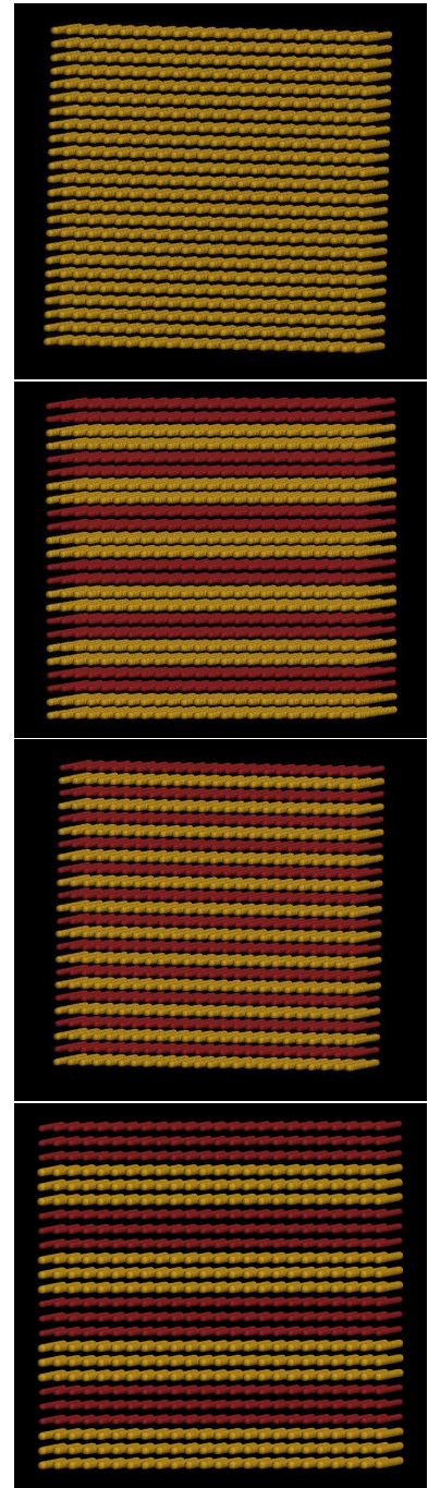
FIG. 1. Ground state in the case where a) D/J = 0.4 , r_c = 2.3 : uniform configuration ; b) D/J = 1 , r_c = 2.3 : double-layer structure; c) D/J = 2 , r_c = 2.3 : single-layer structure; d) D/J = 0.4 , r_c = \sqrt{10} \simeq 3.16 : triple-layer structure. See text for comments.
