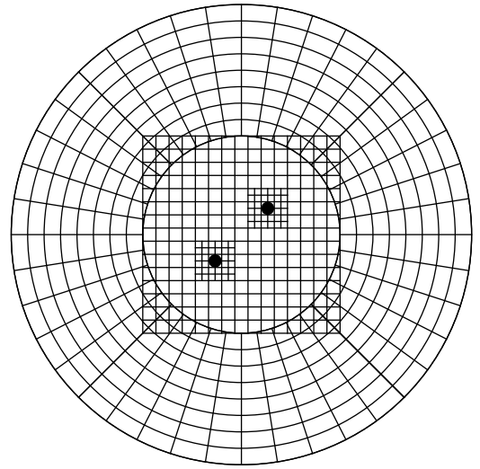
FIG. 1: Schematic diagram of a typical Llama grid setup in the (x, y) plane. Note the inner Cartesian grid with box-in-box AMR which is joined to a 6-patch multiblock structure (only 4 of these patches are shown in the (x, y) plane).
