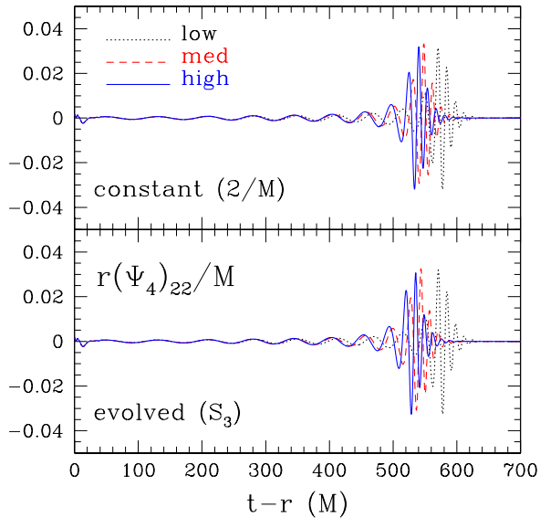
FIG. 6: Real part of the \ell = 2, m = 2 mode of the gravitational waveform \Psi_4 for the unequal-mass black-hole binary. Different lines refer to different resolutions (see text for details) and the two panels refer to the case when \eta is kept constant in space and time (upper panel) or when it is evolved with source given by (14) (lower panel).
