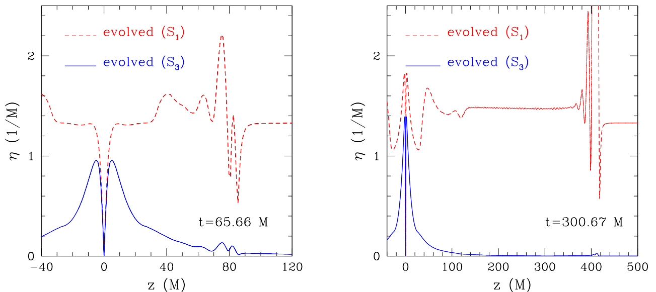
FIG. 4: Profiles along the z -axis of the damping term \eta for an equal-mass BBH system. Different lines refer to the case when \eta evolved with sources given respectively by (12) (red dashed line) or by (13) (blue solid line). The left and right panel refers to two different times and highlight the importance of the fall-off term to avoid reflections at mesh boundaries. Note that the outer boundary is at \simeq 2000 M and cannot be responsible for the appearance of the spikes via reflection.
