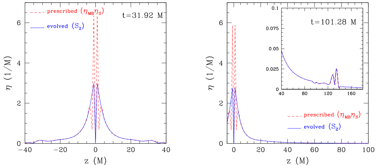
FIG. 3: The same as in Fig. 2, but the prescribed damping term Eq. (5) is tapered with a function Eq. (8), while the source term for the evolution equation is given by (13). Note that in this case the damping term falls off as expected but that in the case of the prescribed \eta_{\text{MB}}(r)\eta_{\text{S}}(r) , the outgoing gauge pulses still produces sharp features near the BH at z \sim 3 M , which do not propagate away. Moreover, sharp features are produced as the initial spikes pass through the interpatch boundaries located at z \sim 40 M . Smoother profiles can instead be obtained by evolving the damping factor.
