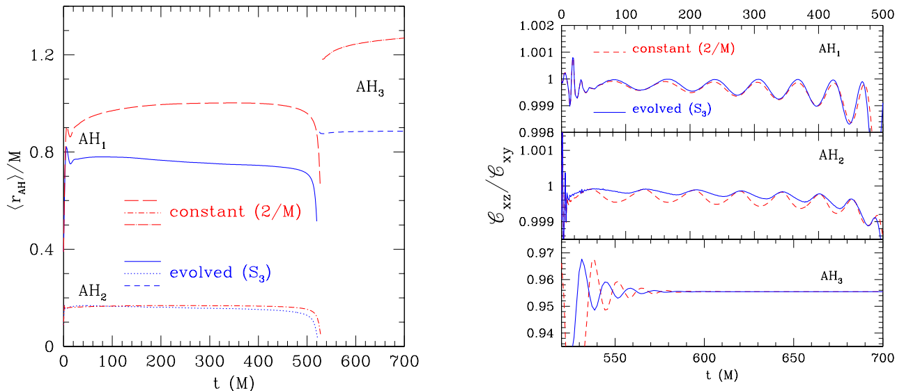
FIG. 8: Left panel: Evolution of the average radius of the AHs on the (x, y) plane before and after the merger. Shown with red long-dashed (large BH), dot-dashed (small BH) and dashed lines (merged BH) are the radii obtained for the case in which \eta is kept constant in space and time. Shown instead with blue solid (large BH), dotted (small BH) and short-dashed lines (merged BH) are the radii obtained for the case in which \eta is evolved with source given by (14). Right panel: Evolution of the ratio of the AHs' proper circumferences on the (x, z) and (x, y) planes, \mathcal{C}_{xz} , \mathcal{C}_{xy} as computed for the three BHs. The first two panels from the top refer to the AHs of the binary, while the bottom one refers to the merged AH and thus covers a different range in time.
