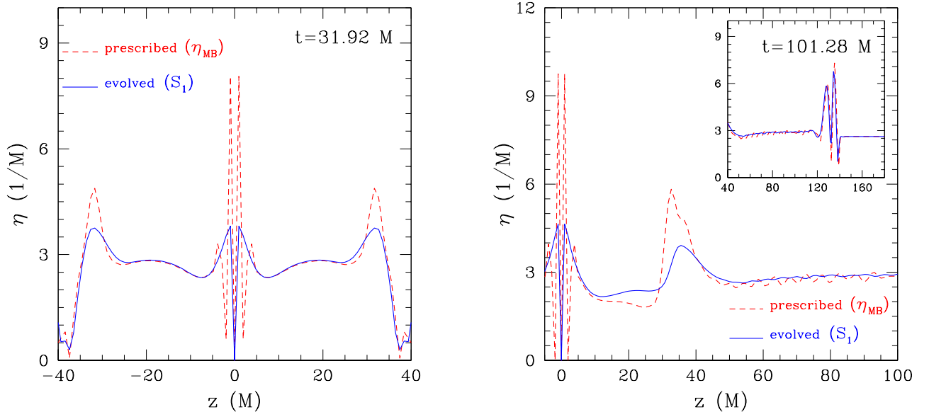
FIG. 2: Profiles along the z -axis of the damping term \eta for an isolated Schwarzschild BH. Different lines refer to the case when \eta is prescribed using Eq. (5) (red dashed line) or when evolved in time using Eq. (9) with source given by (12) (blue solid line). The left panel refers to an earlier time and focuses on the central region of the grid. The right panel refers to a later time and shows a larger portion of the grid, highlighting that in contrast to the dynamical \eta , the evolved one leads to smooth profiles at the patch boundary (see inset). Note that the outer boundary is at 400 M and cannot be responsible for the appearance of the spikes via reflection.
