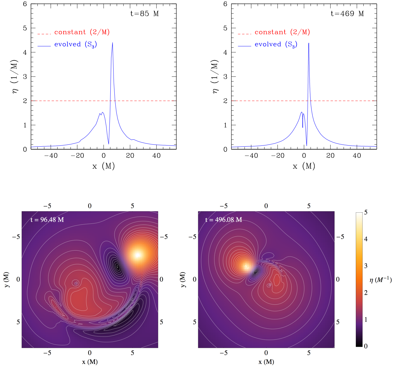
FIG. 5: Spatial dependence of the damping term \eta for an unequal-mass BBH system with q = 1/4 . Different lines refer to the case when \eta is kept constant in space and time (red dashed line) or when it is evolved in time using Eq. (9) with source given by (14) (blue solid line). The top left and right panels refer to two different times when the punctures are close to the x -axis and show that the new gauge drives the damping term to follow the BHs and be smooth elsewhere. The bottom left and right panels, instead, show the damping term on the (x, y) plane at two representative times and show the non trivial but smooth distribution of the damping term which adapts to the motion of the punctures (the latter are near the maxima of the \eta ).
