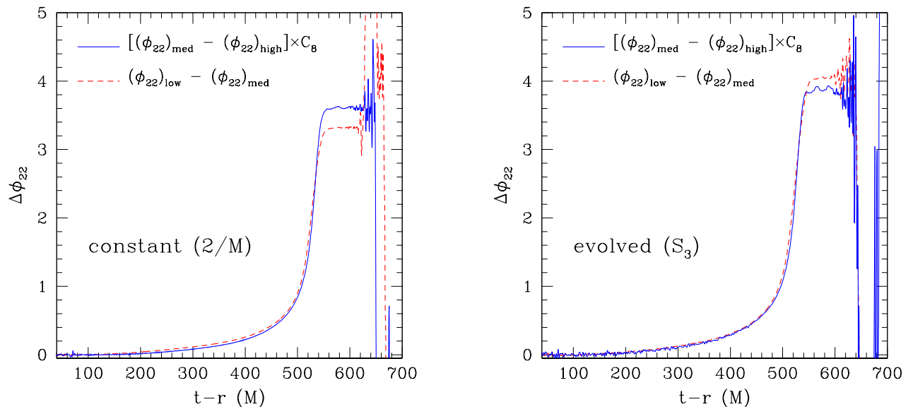
FIG. 7: Phase difference in the \ell = 2, m = 2 mode of the gravitational waveforms as computed between the low and medium resolutions (red dashed line) and between the medium and high resolutions (blue solid line). The latter has been scaled to compensate for an 8th-order convergence which is indeed obtained as shown by the good overlap between the curves. The left panel refers to the case when \eta is kept constant in space and time, while the right one to when it is evolved with source given by (14).
