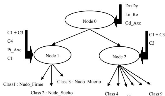
Figure 1: Example of hierarchical description.
