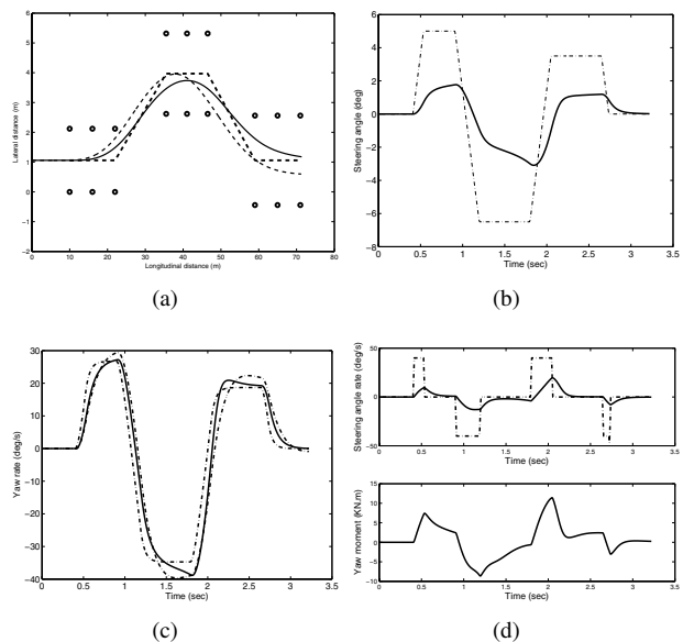
Fig. 4. ISO3888-2 maneuver: Yaw rate, steering angle, steering angle rate and trajectory for the uncontrolled and the controlled vehicles.
