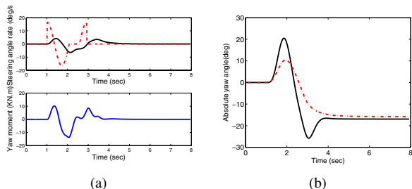
Fig. 7. Sine with dwell maneuver: Steering rate and differential braking control inputs, vehicle absolute yaw angle. Dashed line for the uncontrolled vehicle and solid line for the controlled one.
