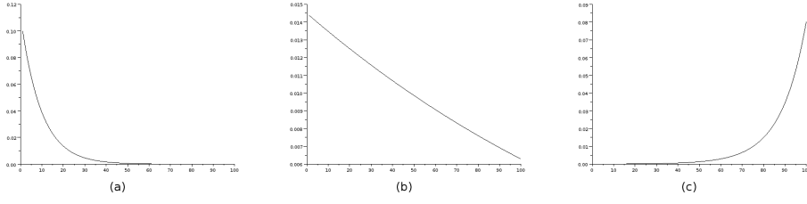
Figure 2: Example 2. Yaglom limits for different values of \lambda . The following values of \theta(\alpha) are obtained by numerical computation. (a) \lambda = 0.9 , \theta(\alpha) = 0.100 ; (b) \lambda = 1.0 , \theta(\alpha) = 0.014 ; (c) \lambda = 1.1 , \theta(\alpha) = 5.84 \times 10^{-5} .
