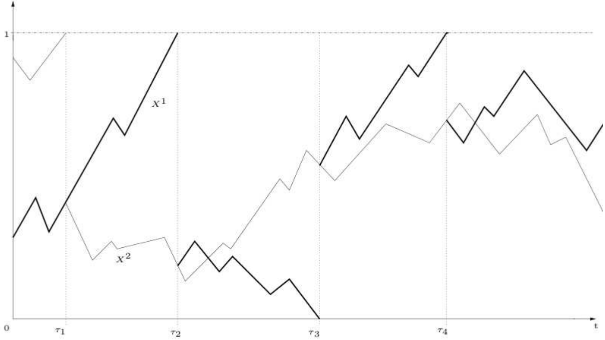
Figure 12: Fleming-Viot type system with two particles absorbed in 0 and 1.
