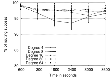
Fig. 13. Average routing success rate
