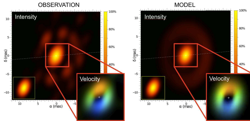
Fig. 5 The VLTI observations of the A[e] system HD62623 (here, the figure of the press release) showed that the dense circumbinary disk (Meilland et al., 2010, outer red ring in both the image – left – and the model – right) seems constantly fed by an inner plasma disk (central yellow dot), probably in Keplerian rotation (insets), whose angular momentum originates from a solar mass companion (Millour et al., 2011).
