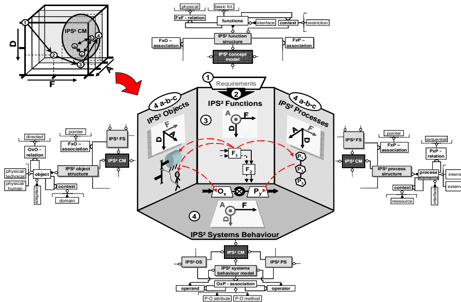
Figure 5 Structure of the extended heterogeneous IPS 2 concept modelling approach (Welp et al. 2008)
