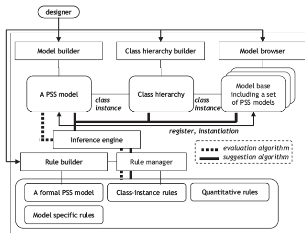
Figure 2 The architecture of Service CAD (Komoto and Tomiyama, 2009)
