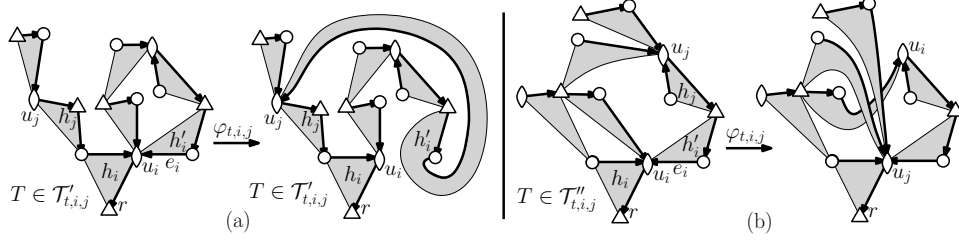
FIGURE 5. The bijection \varphi_{t,i,j} applied to a tree-rooted constellation in \mathcal{T}'_{t,i,j} (left), or in \mathcal{T}''_{t,i,j} (right). The tree-rooted k -constellations are represented as k -hypergraphs together with a rotation system (so the overlappings of the hyperedges in this figure are irrelevant).
