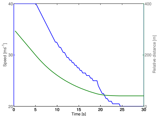
Fig. 9. Fast vehicle approaching scenario
