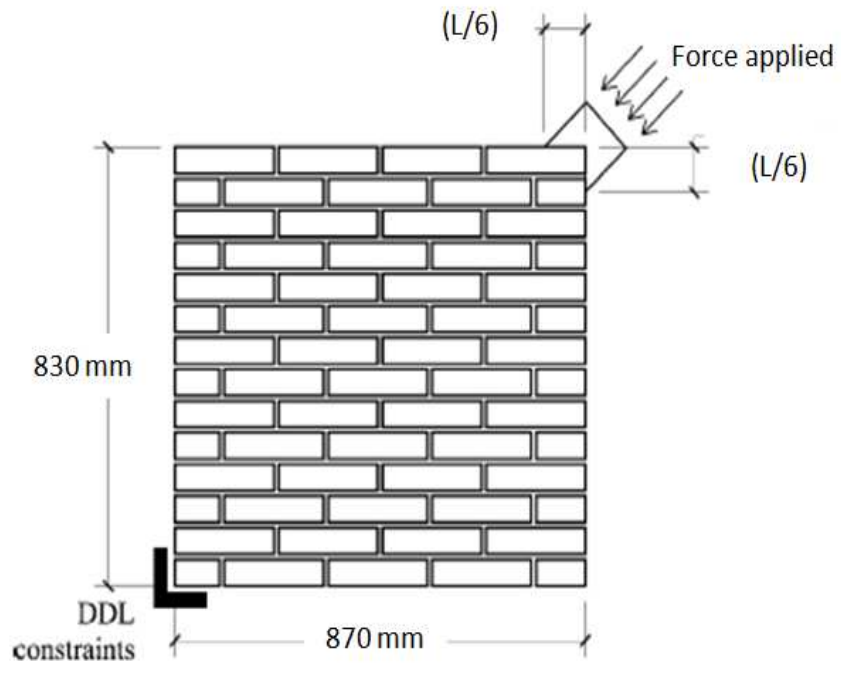
Figure 11: Initial geometrical configuration and loading conditions imposed on the wall.
