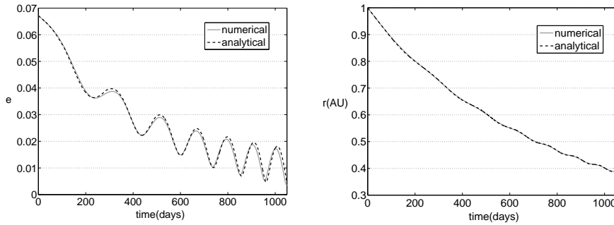
Fig. 7 Comparison between analytical and numerical solution for an Earth to Mercury transfer. The analytical formulas are here rectified three times per orbital revolution
