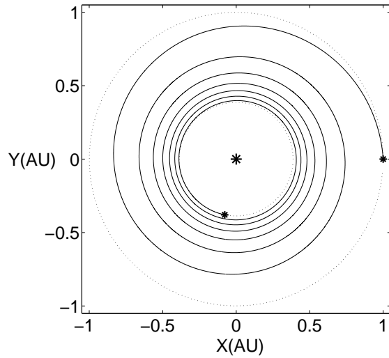
Fig. 6 Low thrust Earth-Mercury orbit transfer. Planets orbits are assumed coplanar and circular for simplicity. The small difference between the numerical and analytical trajectory cannot be appreciated from this plot.
