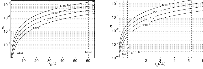
Fig. 1 Variability of the parameter epsilon for Earth (right) and interplanetary orbits (left)
