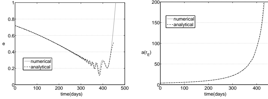
Fig. 5 Comparison between analytical and numerical solution for an orbit raising maneuver from GTO to earth escape. The plotted quantities are the orbit eccentricity (left) and semimajor axis (right). The analytical formulas are propagated twice per orbital revolution.
