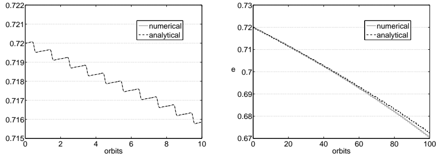
Fig. 3 Comparison between analytical and numerical solution for the evolution of the eccentricity in a GTO orbit raising maneuver.
