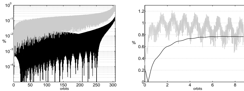
Fig. 4 Percentage of phasing (dark) and position error (grey) of the analytical solution for the GTO orbit raising (left) and the Mercury transfer (right).
