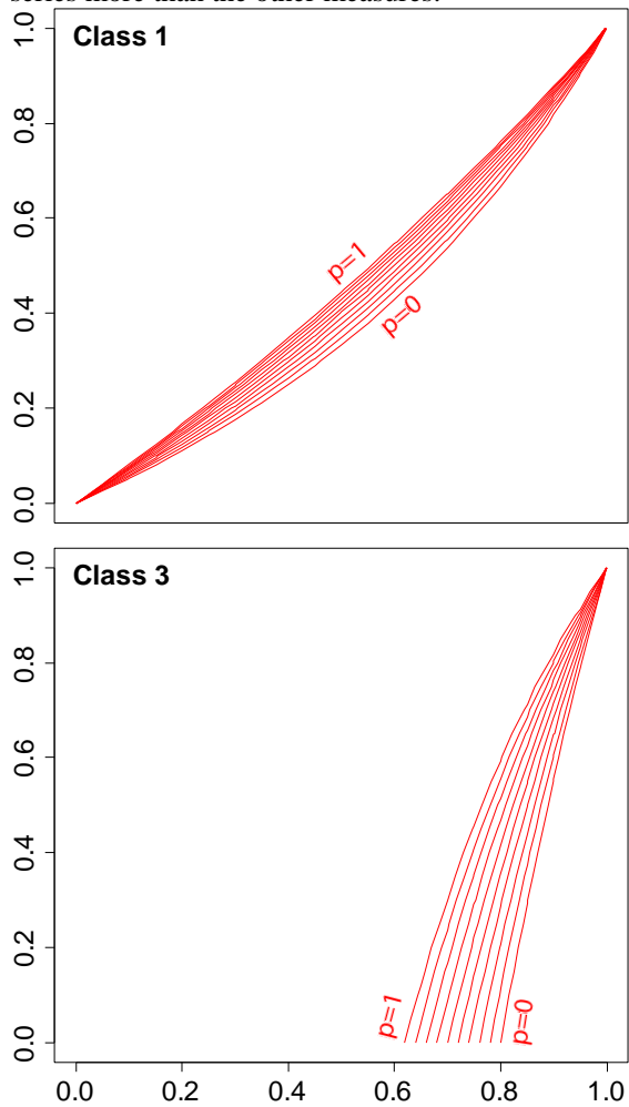
Figure 3: Discrimination lines of the F-measure for classes 1 (top) and 3 (bottom), with k=3 .
