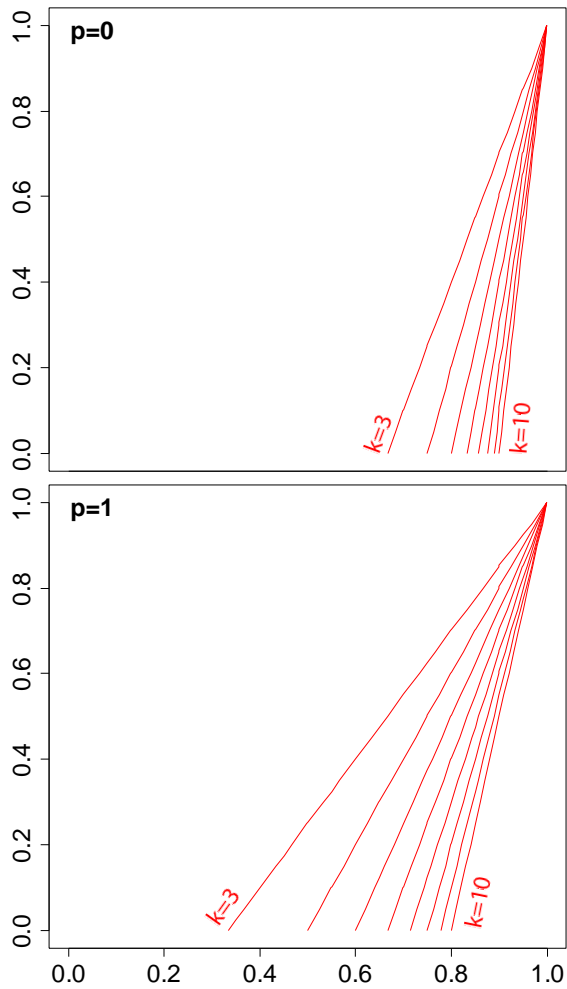
Figure 5: Discrimination lines of OSR for p=0 (top) and p=1 (bottom), with k \in [3;10] .
