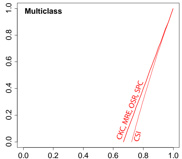
Figure 2: Discrimination lines of all multiclass measures, with p=0 and k=3 .
