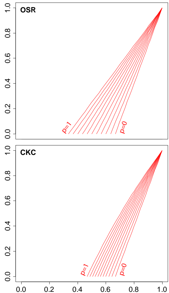
Figure 4: Discrimination lines of OSR (top) and CKC (bottom), with k=3 .
