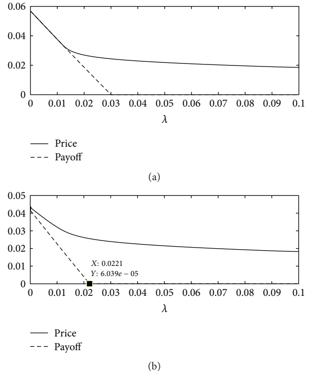
FIGURE 9: The price of the prepayment option P_{\Lambda}(\lambda) (solid line) and the payoff \chi(\lambda) (dashed line) as function of the intensity \lambda . (a) regime X = e_1 ; (b) regime X = e_2 . Two regions appear: the continuation region \lambda > \Lambda_1^* and the exercise region \lambda \leq \Lambda_1^* . For the second regime there is no exercise region.
