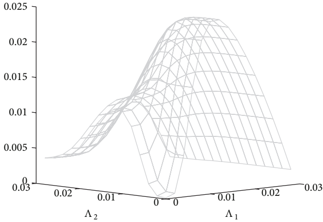
FIGURE 7: We illustrate here the dependence of P_{\Lambda}(\bar{\lambda}_0, \bar{X}_0) as a function of the exercise boundary \Lambda ; this allows to find the optimal (\Lambda_1^* = 121 \text{ bps}, \Lambda_2^* = 0) that maximizes the option price.
