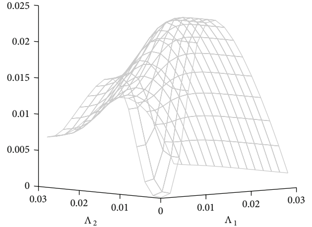
FIGURE 4: We illustrate here the dependence of P_\Lambda(\bar{\lambda}_0, \bar{X}_0) as a function of \Lambda ; this allows for finding the optimal ( \Lambda_1^* = 122 bps, \Lambda_2^* = 64 bps) that maximizes the option price.
