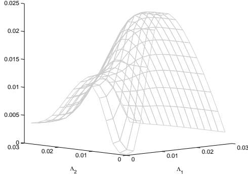
FIG. 3.4. We illustrate here the dependence of P_{\Lambda}(\bar{\lambda}_0, \bar{X}_0) as a function of the exercise boundary \Lambda ; this allows to find the optimal ( \Lambda_1^* = 121bps, \Lambda_2^* = 0 ) that maximizes the option price.
