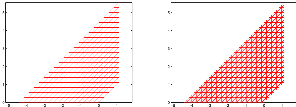
FIGURE 21. Meshes M16S (384 triangles) and M32S (1536 triangles).
