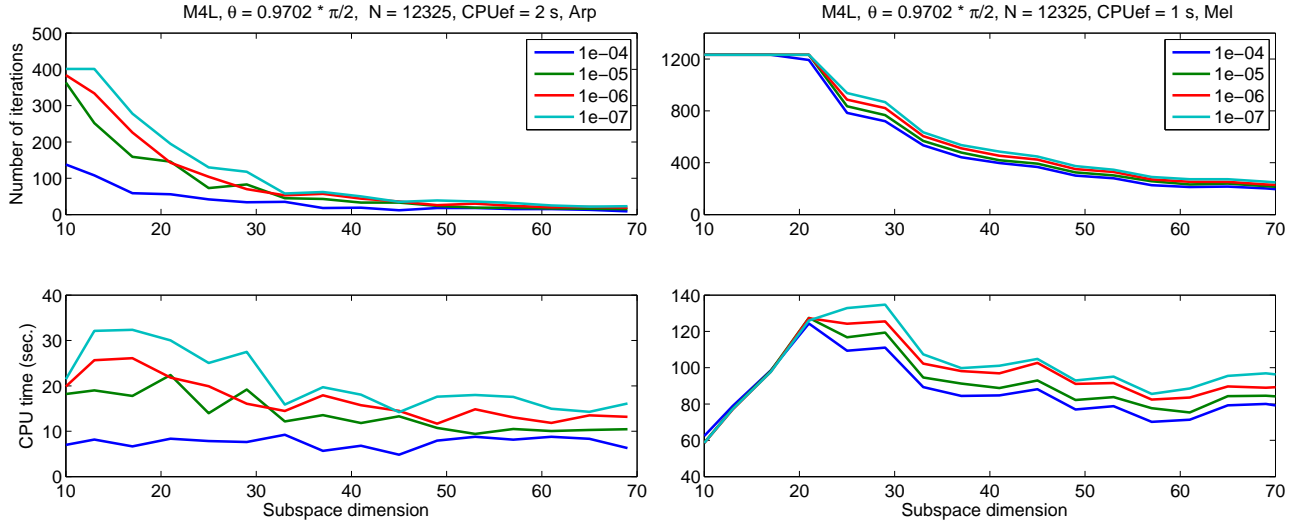
FIGURE 18. Comparison of the behavior of the methods for the large angle \theta = 0.9702 * \pi/2 .
