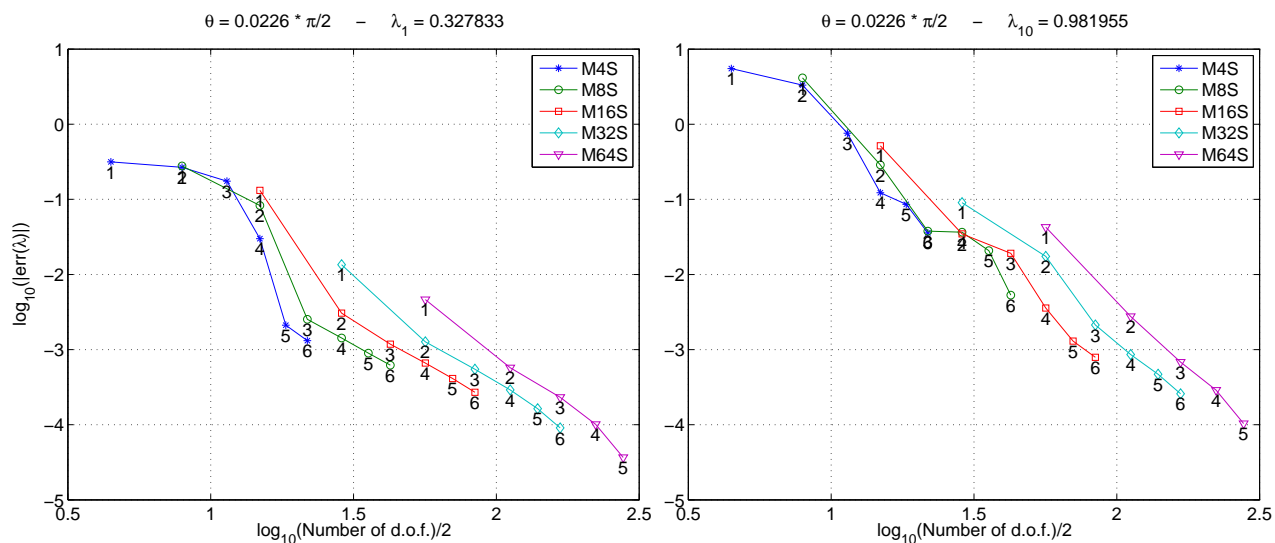
FIGURE 22. Convergence towards \lambda_1 \simeq 0.32783 and \lambda_{10} \simeq 0.98195 .
