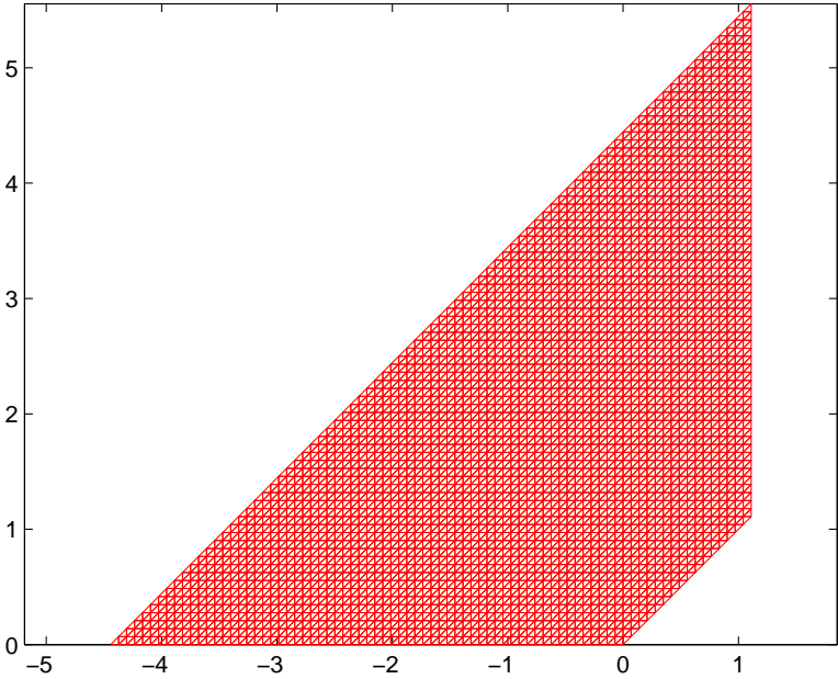
FIGURE 17. Mesh M64S for small angle, 6144 triangles.
