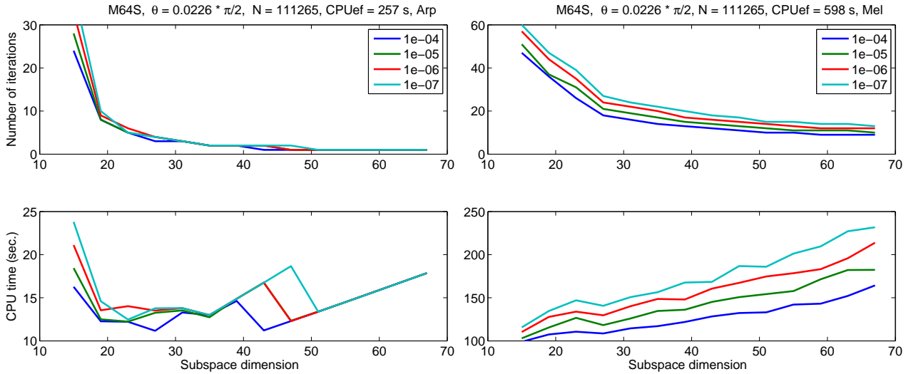
FIGURE 19. Comparison of the behavior of the methods for the small angle \theta = 0.0226 * \pi/2 .
