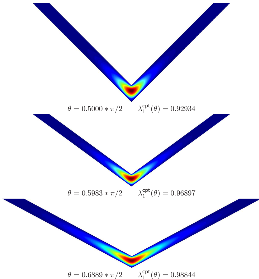
FIGURE 8. Computations for moderately large angles. Plots of the first eigenvectors in the physical domain (rotated by \frac{\pi}{2} ). Numerical value of the corresponding eigenvalue \lambda_1(\theta) .
