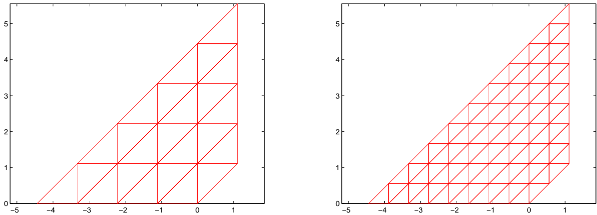
FIGURE 20. Meshes M4S (24 triangles) and M8S (96 triangles).
