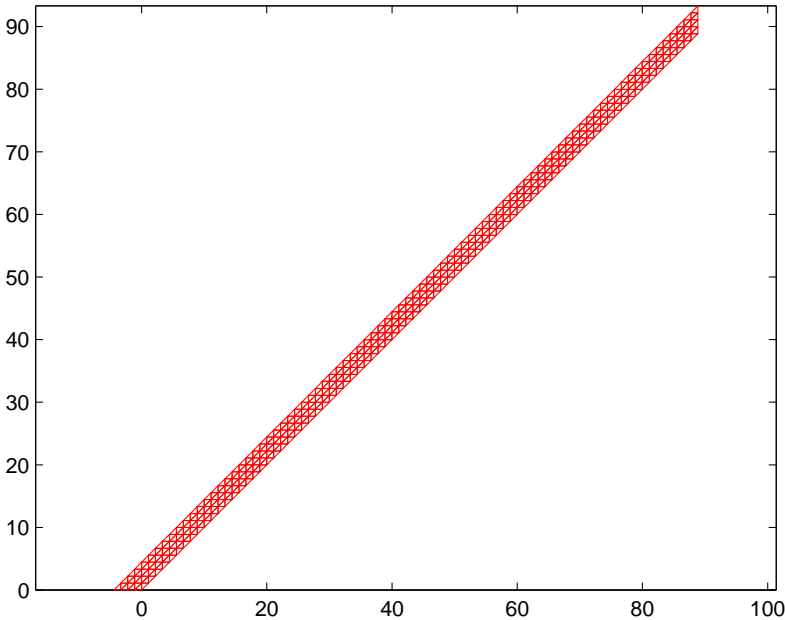
FIGURE 16. Mesh M4L for large angle, 656 triangles.
