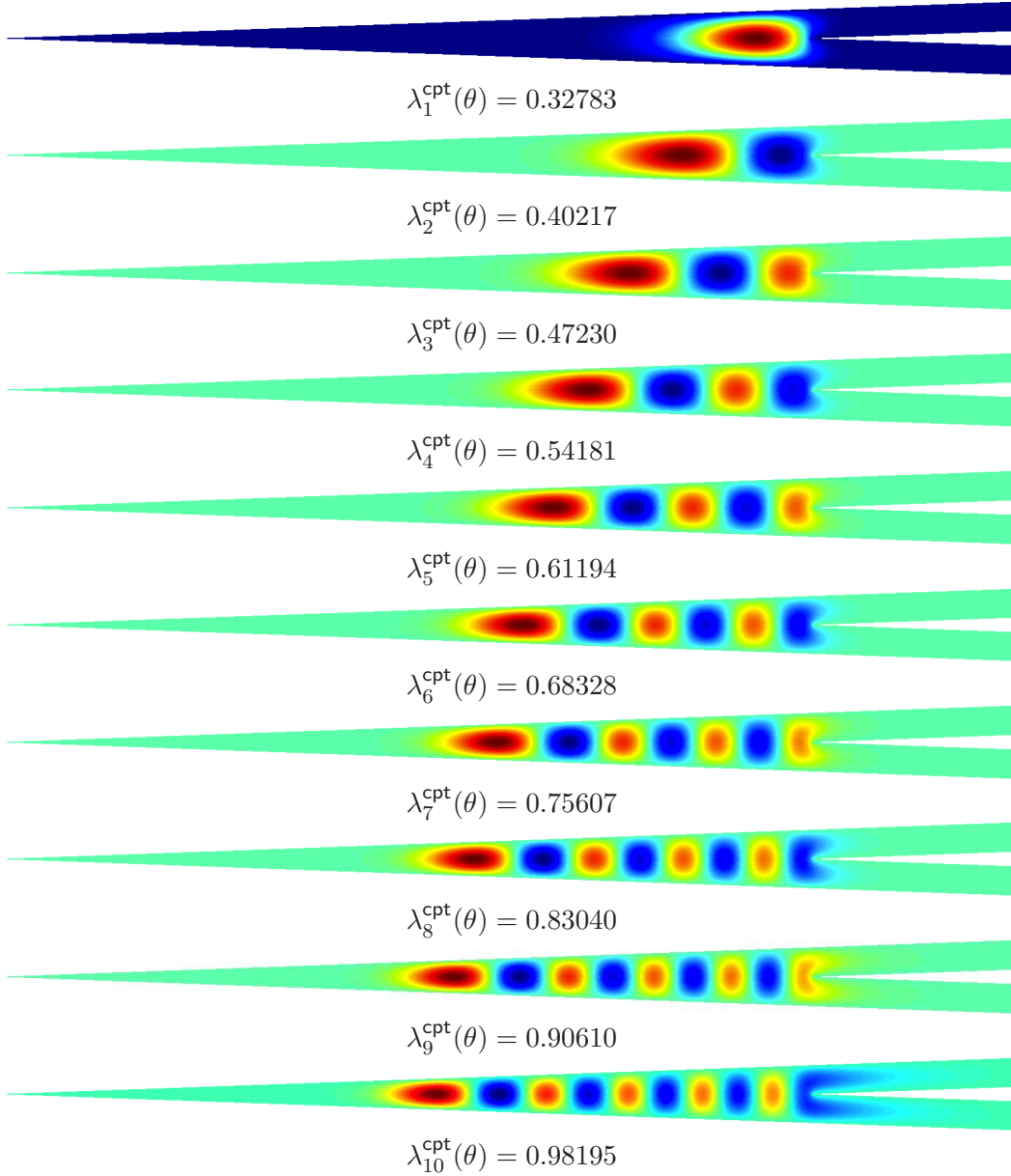
FIGURE 11. Computations for \theta = 0.0226 * \pi/2 \sim 2^\circ with the mesh M64S (see Figure 17). Numerical values of the 10 eigenvalues \lambda_j(\theta) < 1 . Plots of the associated eigenvectors in the physical domain.
