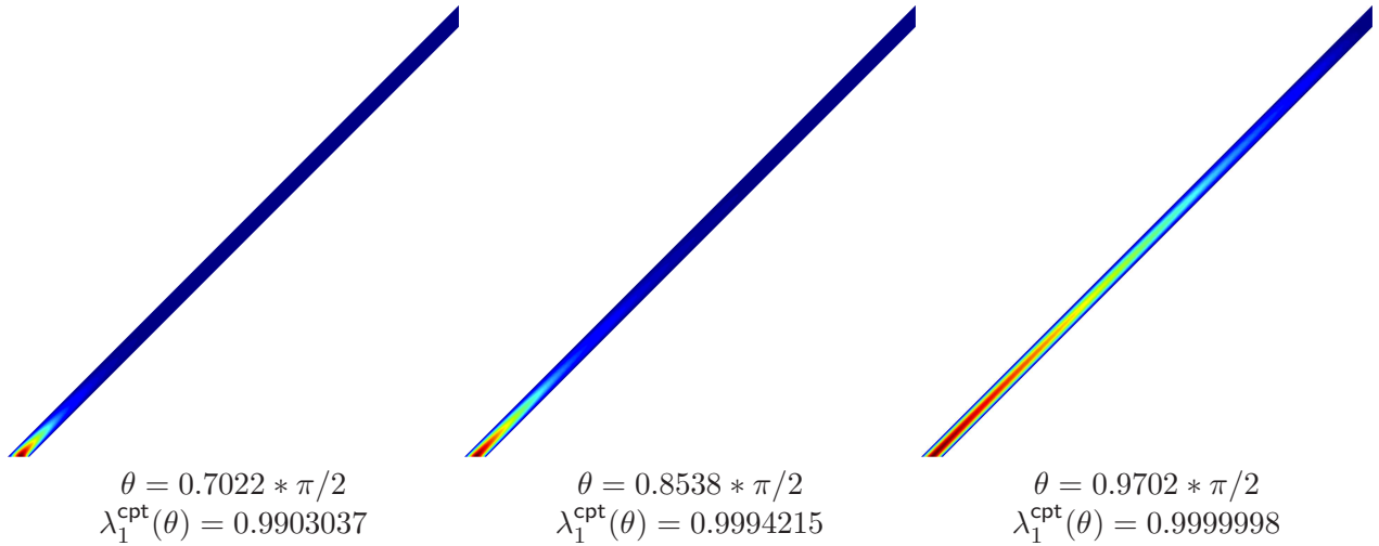
FIGURE 9. Computations for very large angles with the mesh M4L (see Figure 16). Plots in the computational domain \Omega .
