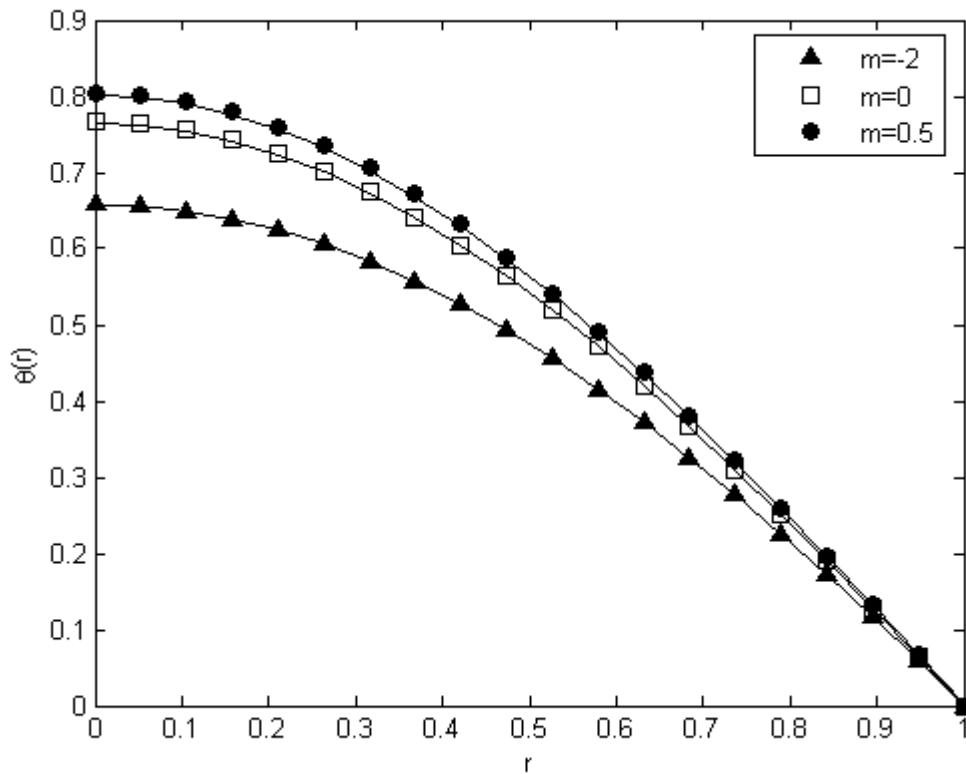
Figure 3. Comparison of sphere numerical and HPM results of the boundary value problem (3-4) for \varepsilon = 0.1 , \delta=2.8 . Solid lines: Numerical solutions; Symbols: HPM solutions.
