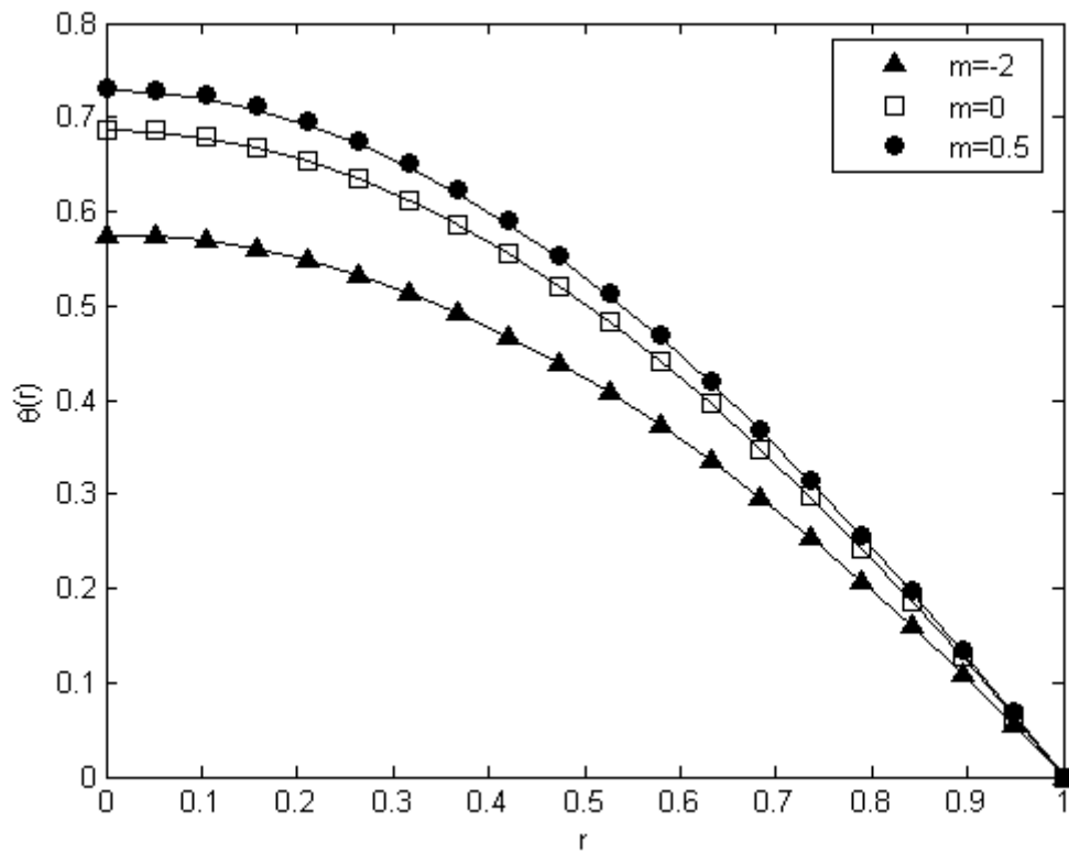
Figure 1. Comparison of slab numerical and HPM results of the boundary value problem (3-4) for \varepsilon = 0.1 , \delta = 0.5 . Solid lines: Numerical solutions; Symbols: HPM solutions.
