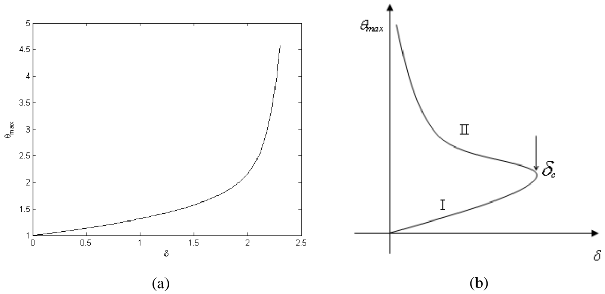
Figure 6. \theta_{\max} versus \delta ; (a) calculated, (b) expected form.
