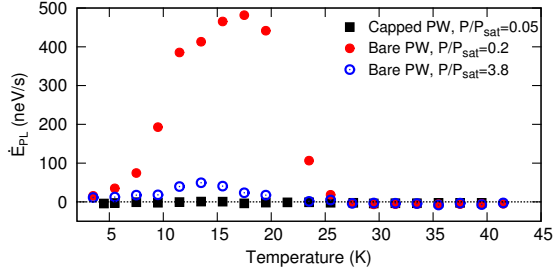
FIG. 2. (Color online) \dot{E}_{\text{PL}} as a function of T for excitation power P/P_{\text{sat}} = 0.2 ( \bullet ) and P/P_{\text{sat}} = 3.8 ( \odot ) in a bare PW and for P/P_{\text{sat}} = 0.05 in a capped PW ( \blacksquare )
