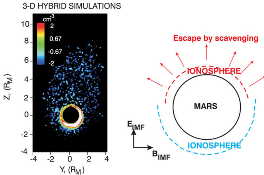
Fig. 8. Map of the \text{O}^+ number density in the Y_{\text{IMF}}Z_{\text{IMF}} plane near the terminator obtained from hybrid simulations. In white bins the number densities are above 10^2 \text{ cm}^{-3} .
