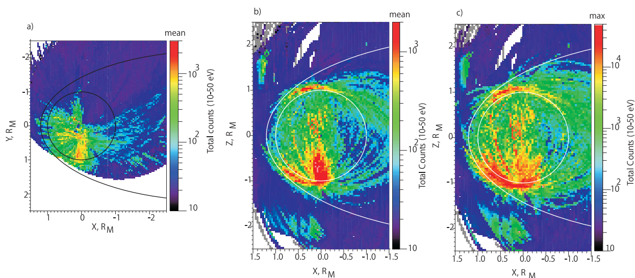
Fig. 10. (a) Map of the proxy ionosphere inferred from the observations of ionospheric oxygen ions in the XY_{MSO} plane obtained from the ASPERA-3 data during almost 3 years of the observations. Strong asymmetry is caused by the fact that the dawn ionosphere was sampled at much higher altitudes than the ionosphere at the dusk side. (b, c) Maps of mean and maximum numbers of counts of low-energy oxygen ions in the XZ_{MSO} plane. Strong asymmetry between the northern and southern ionospheres appears due to the crustal magnetic field. Note that the high fluxes measured in the solar wind are mainly due to the UV contamination.
