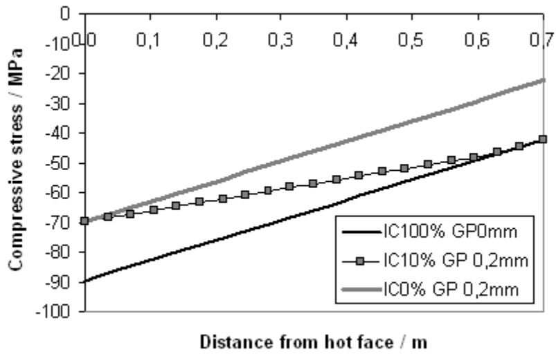
Fig. 7 Stress perpendicular to the joint surface in the model of fig. 2.c. Hot face temperature is 850 °C.
