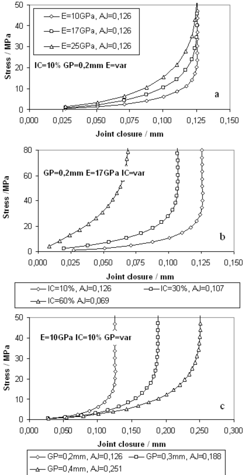
Fig. 6 Joint closure curves calculated by the model of fig. 2b. The effects of brick stiffness (a), initial contact area between the bricks (b), initial contact gap (c).
