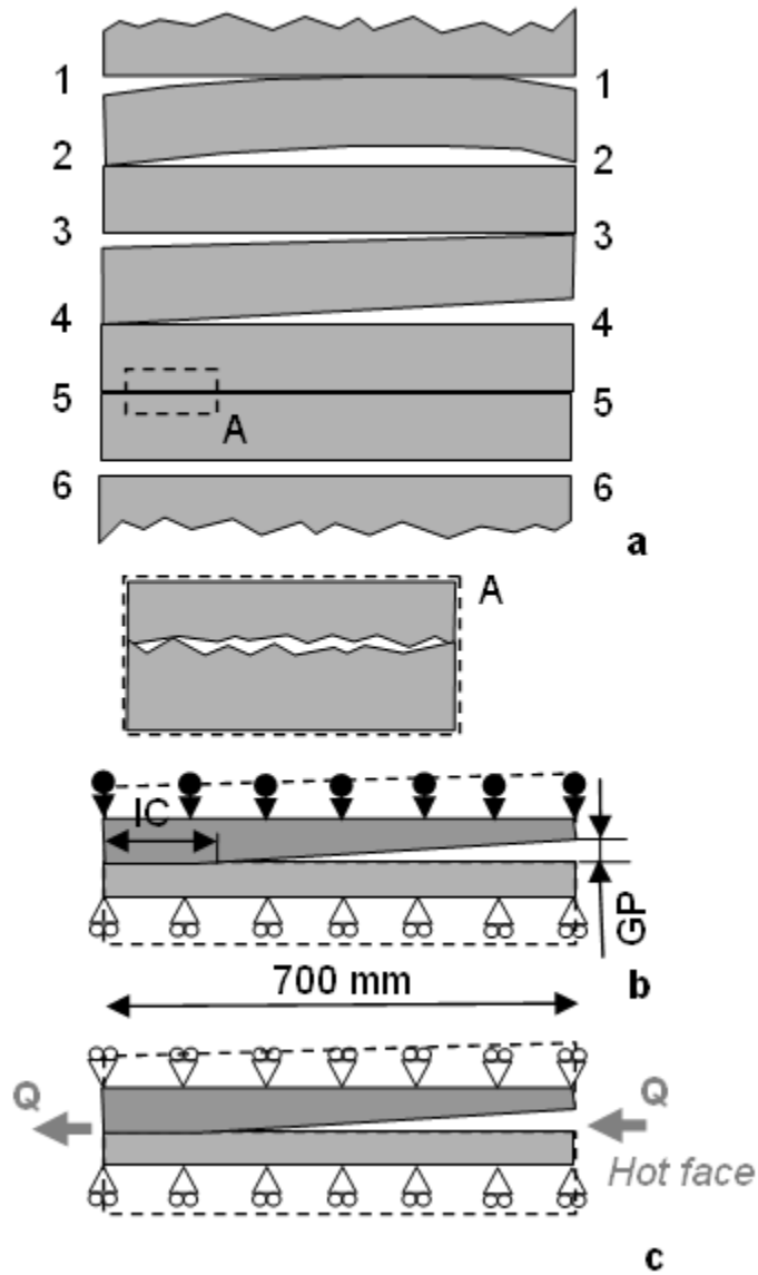
Fig. 2 Possible joint types (a) and FEM model of the joint 4-4 (b, c). The models simulate (b) external displacement loads, (c) own thermal loads.
