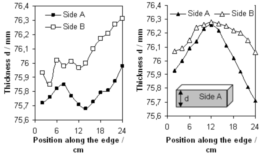
Fig. 5 Typical brick thickness variation for two magnesia-chromite bricks. Sides A and B are opposite each other.
