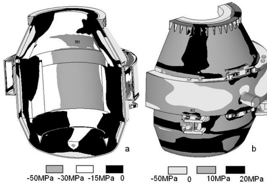
Fig. 1 FEM model of BOF converter showing circumferential stresses in the lining (a) and the shell (b).
