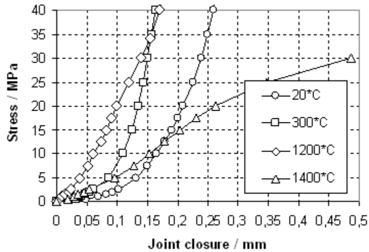
Fig. 4 Joint closure curves of Magnesia-Chromite brick.
