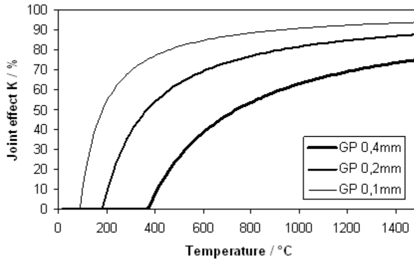
Fig. 8 Reduction of the stress due to joint closure (IC=10%). Stress near the hot face is presented.
