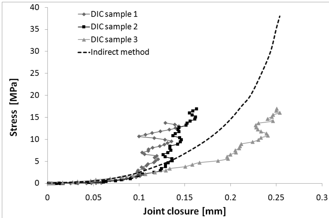
Fig. 3 Comparison of joint closure for the indirect and direct methods at room temperature (MaC, three samples for DIC method, average curve for indirect method).
