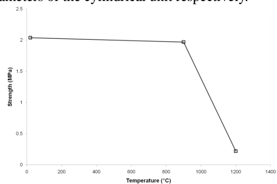
Figure 2: Tensile strength versus temperature for specimen B
