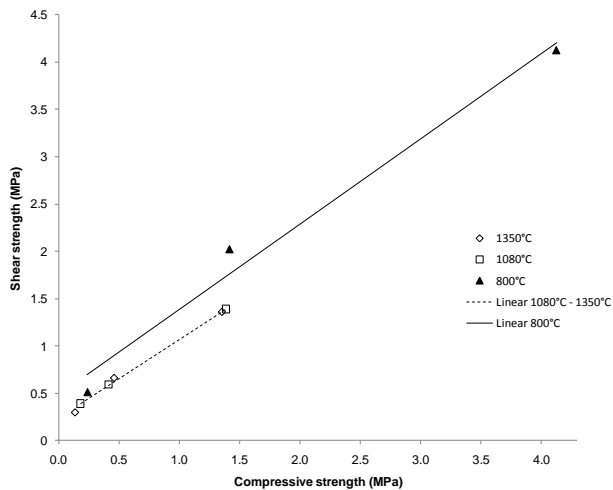
Figure 5: Mohr-Coulomb line for specimen A.
