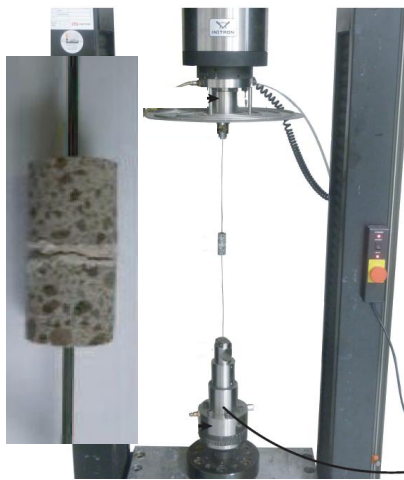
Figure 1: High temperature tensile test set-up
