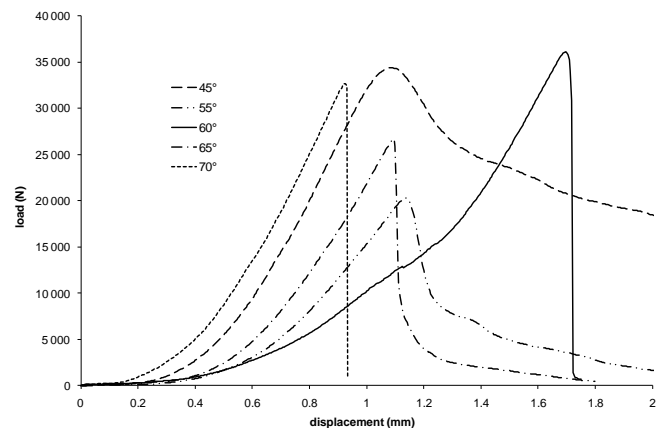
Figure 4: Load versus displacement curves for specimen B with different joint slopes at 900°C
