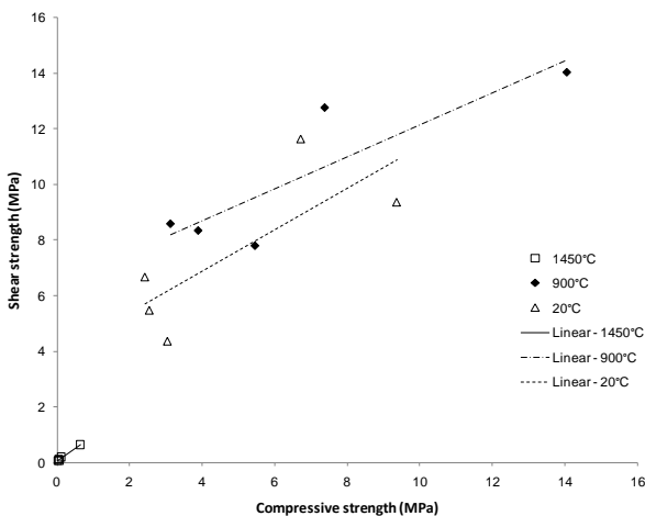
Figure 6: Mohr-Coulomb line for specimen B.
